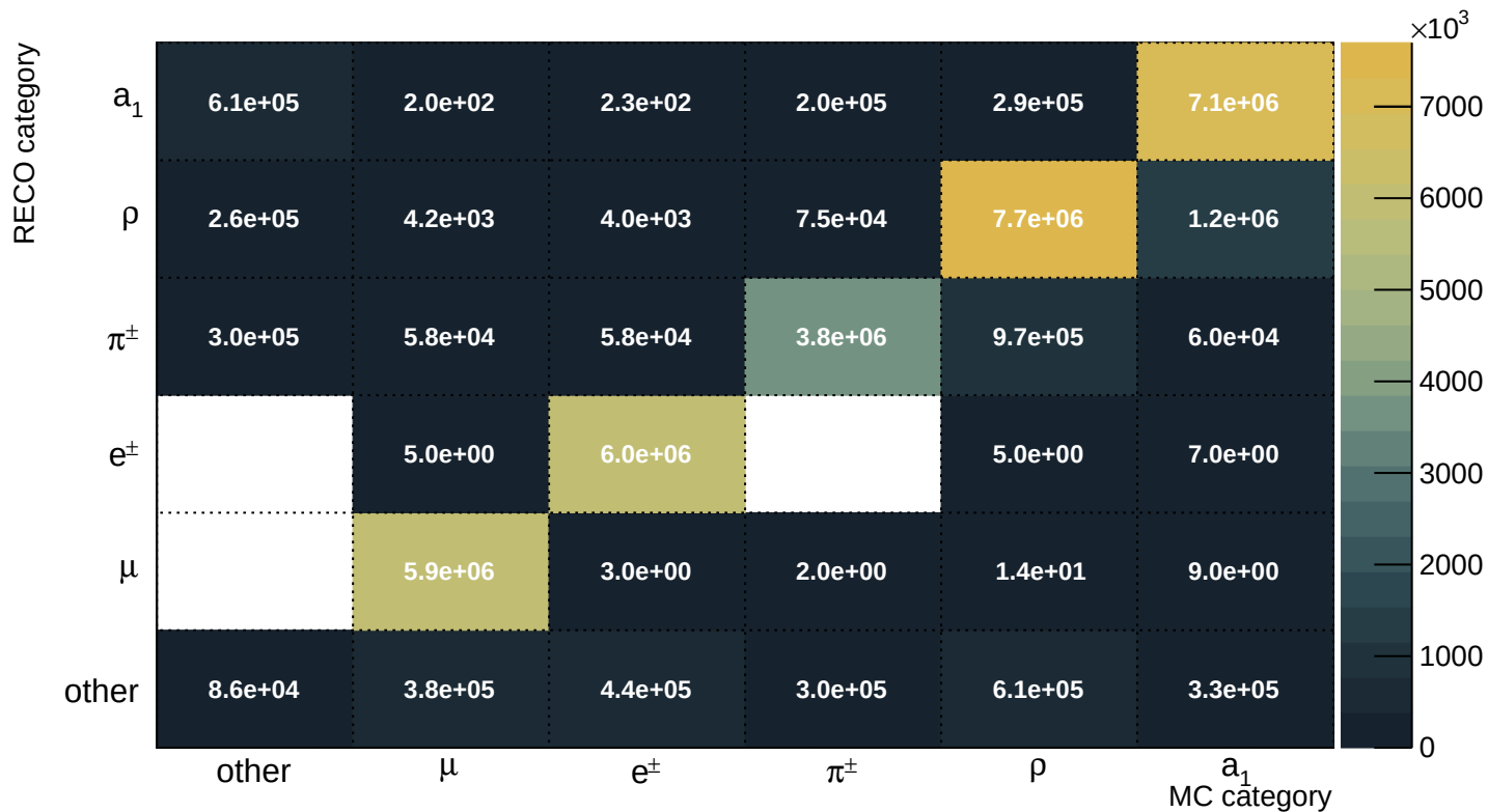
Confusion matrix
