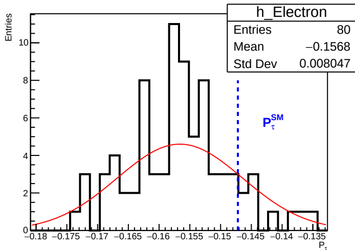
Electron Channel
