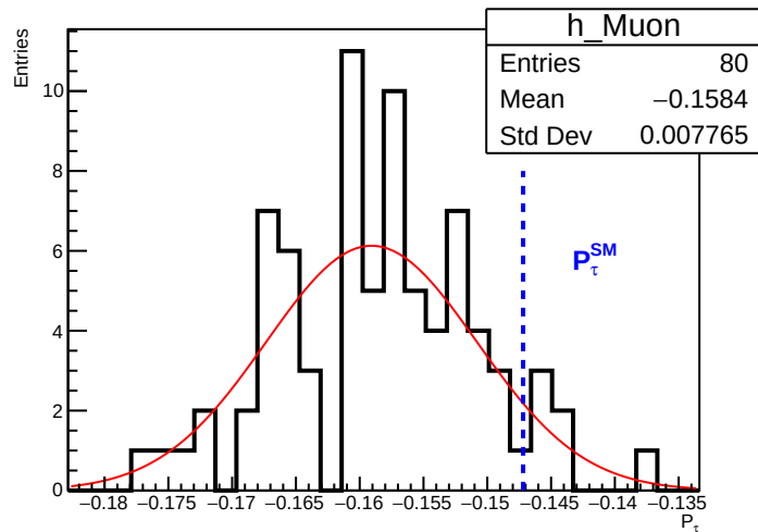
Muon Channel
