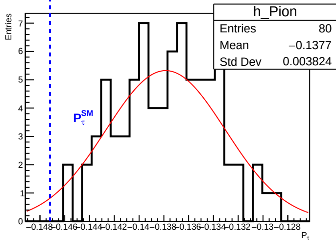
Pion Channel
