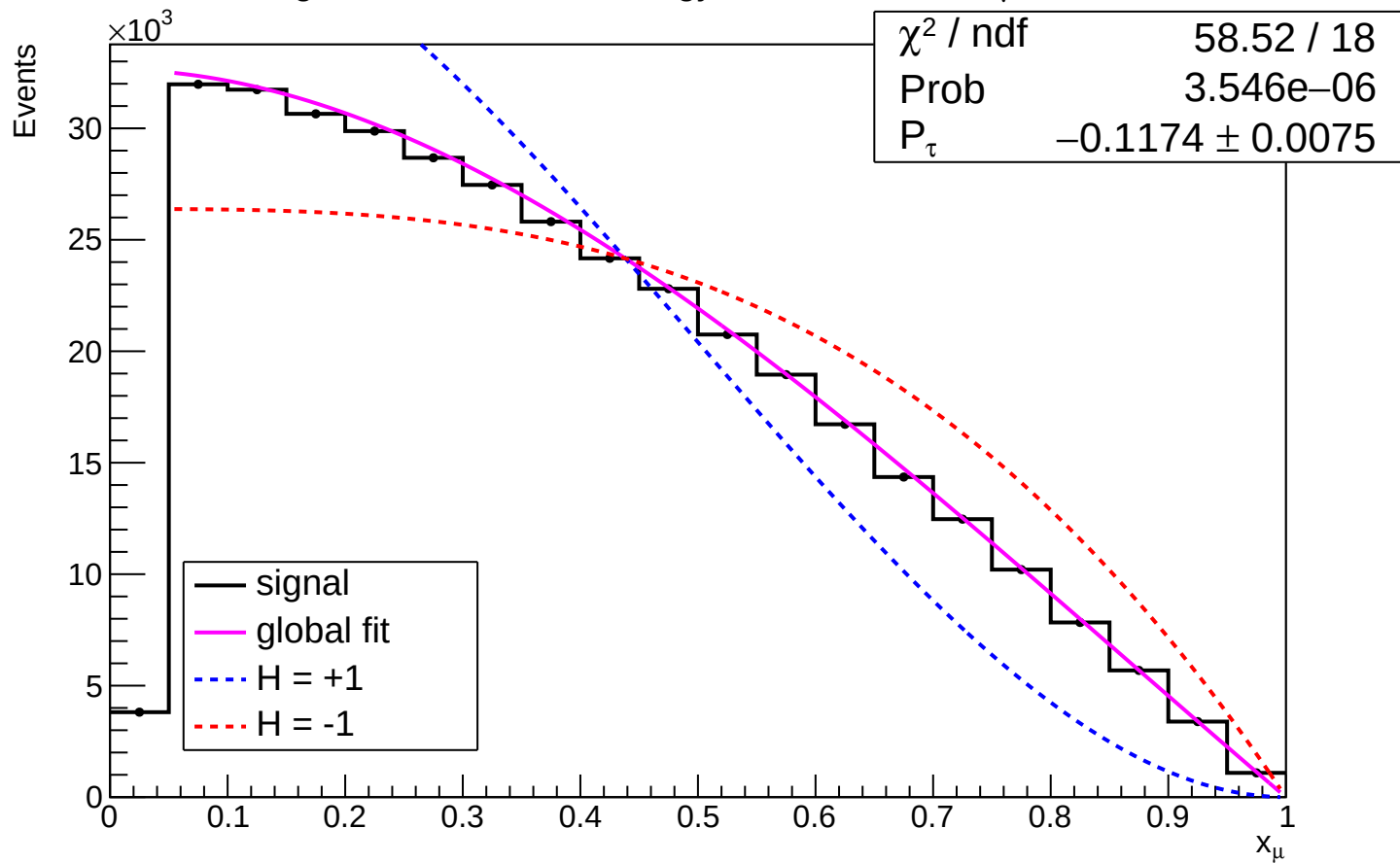
Diagonal events + MC energy + inv mass limit : \mu channel
