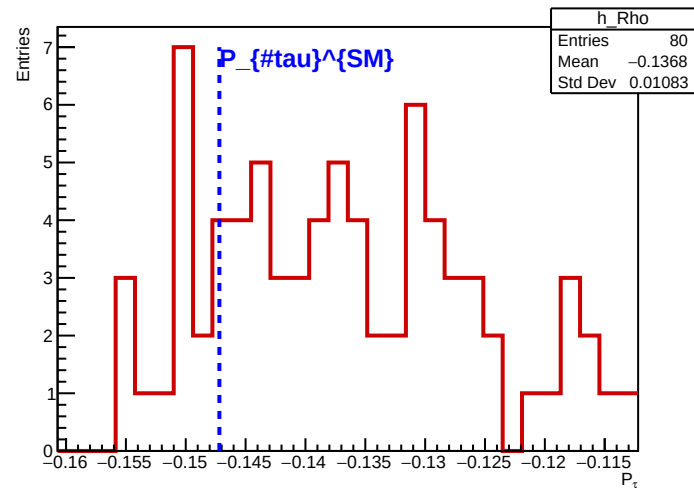
Rho Channel
