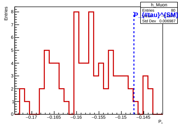
Muon Channel
