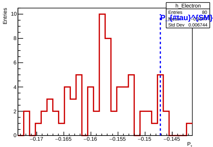
Electron Channel
