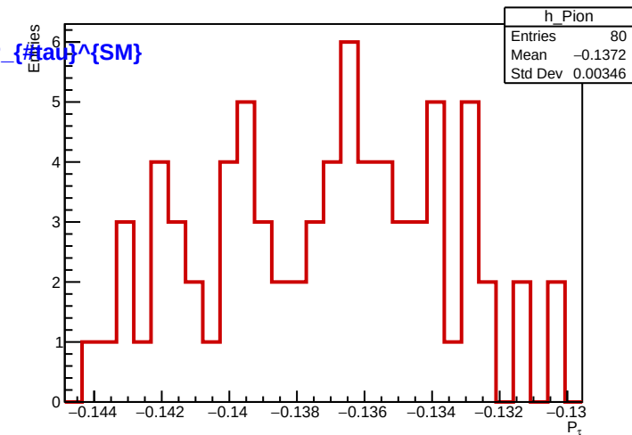
Pion Channel
