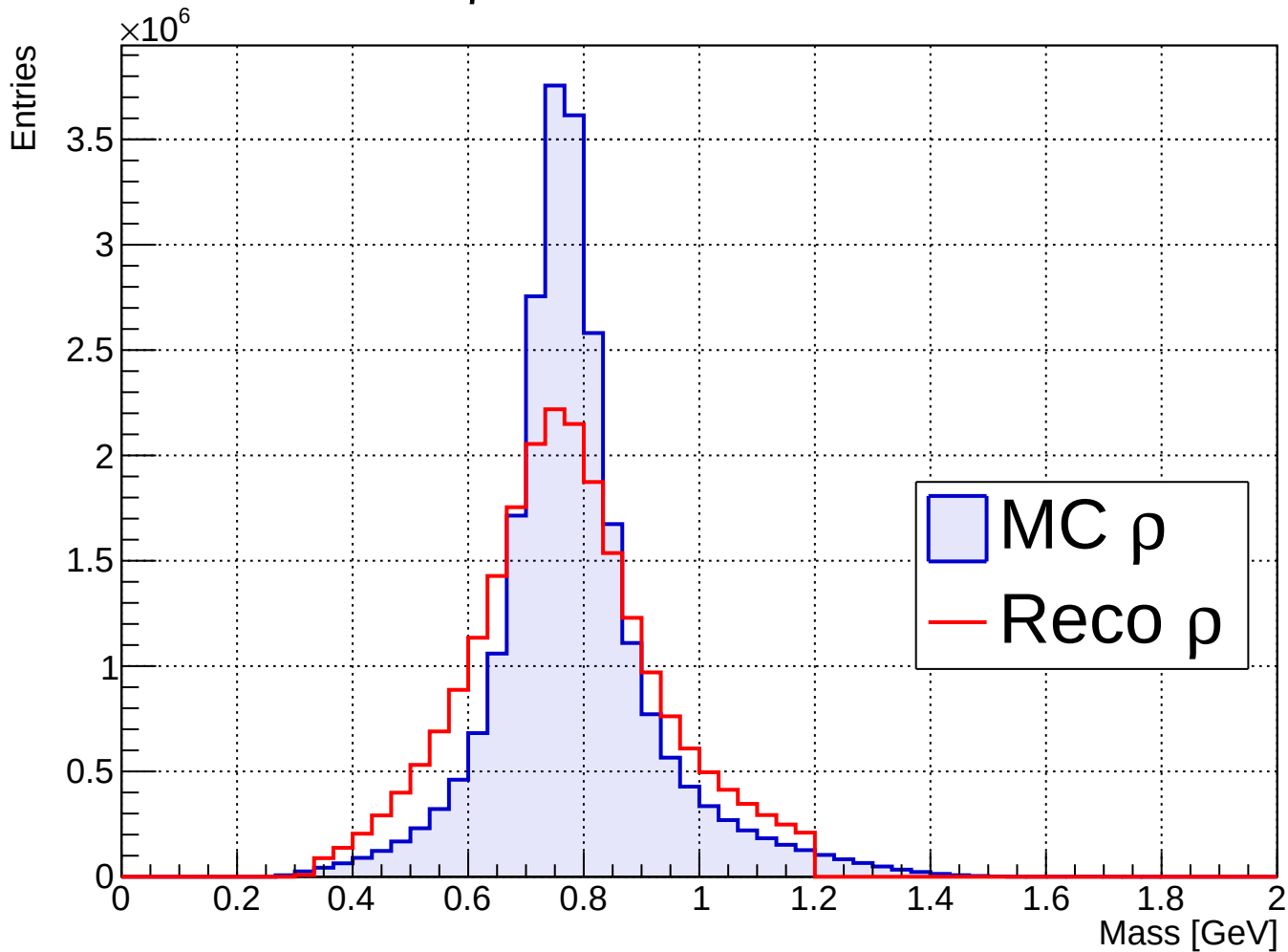
\rho Mass: MC vs Reco
