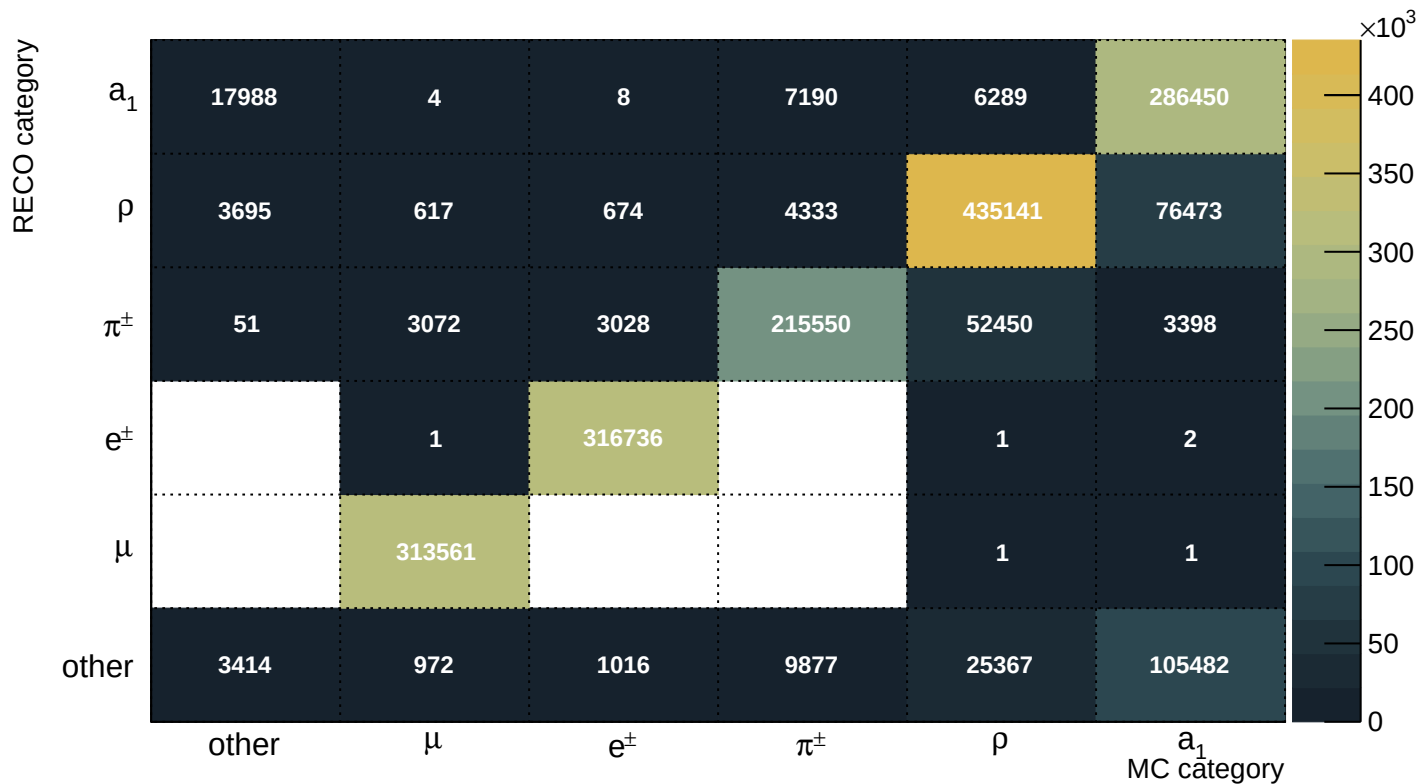
Confusion matrix
