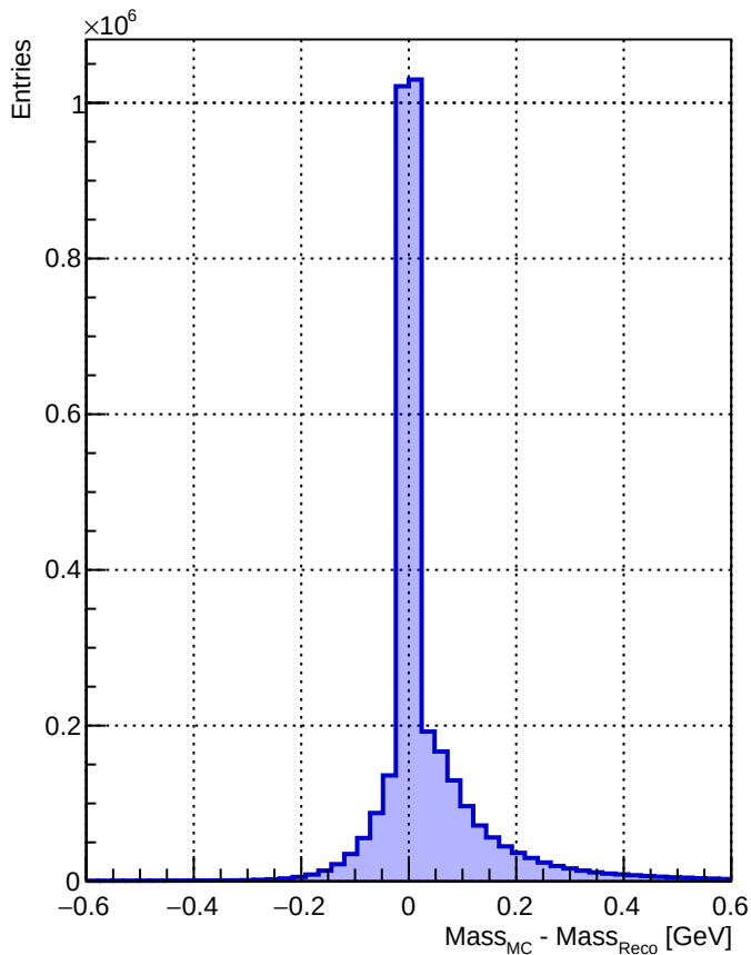
a_1 mass pull
