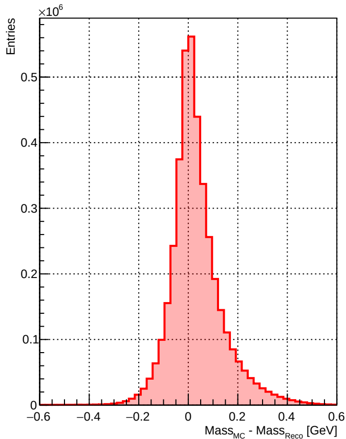
\rho mass pull
