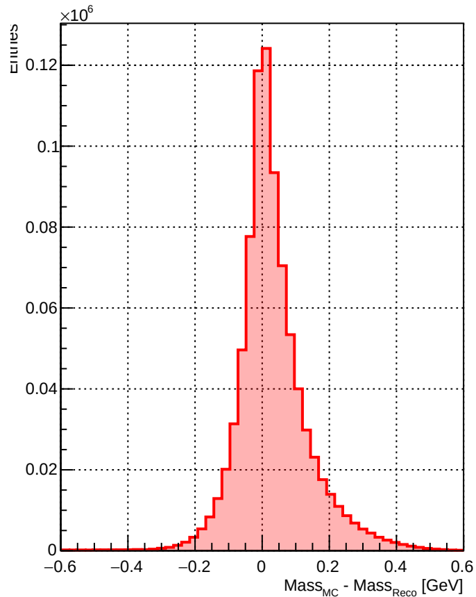
\rho mass pull
