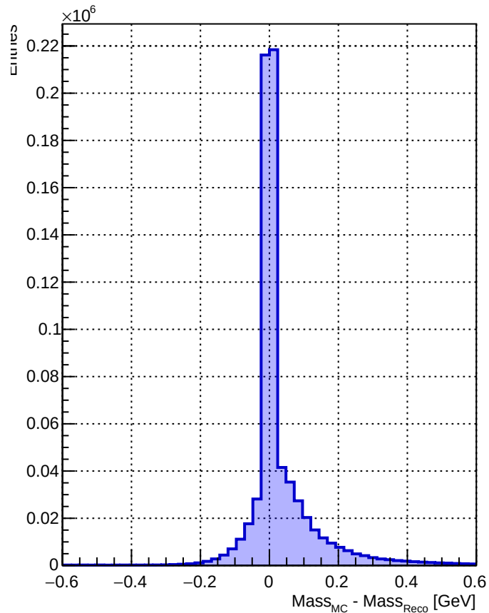
a_1 mass pull
