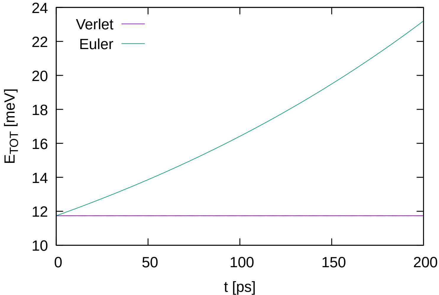
Euler VS Verlet energy conservation
