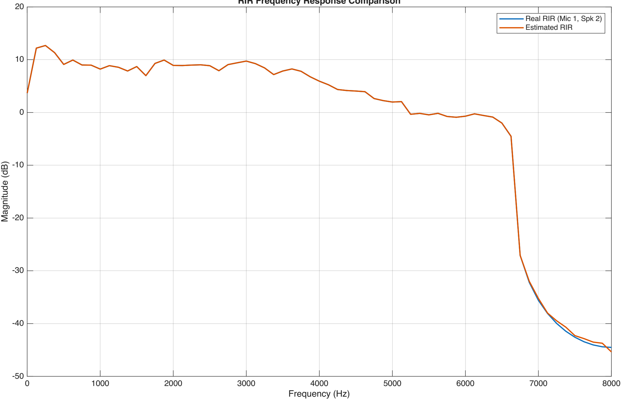
RIR Frequency Response Comparison
