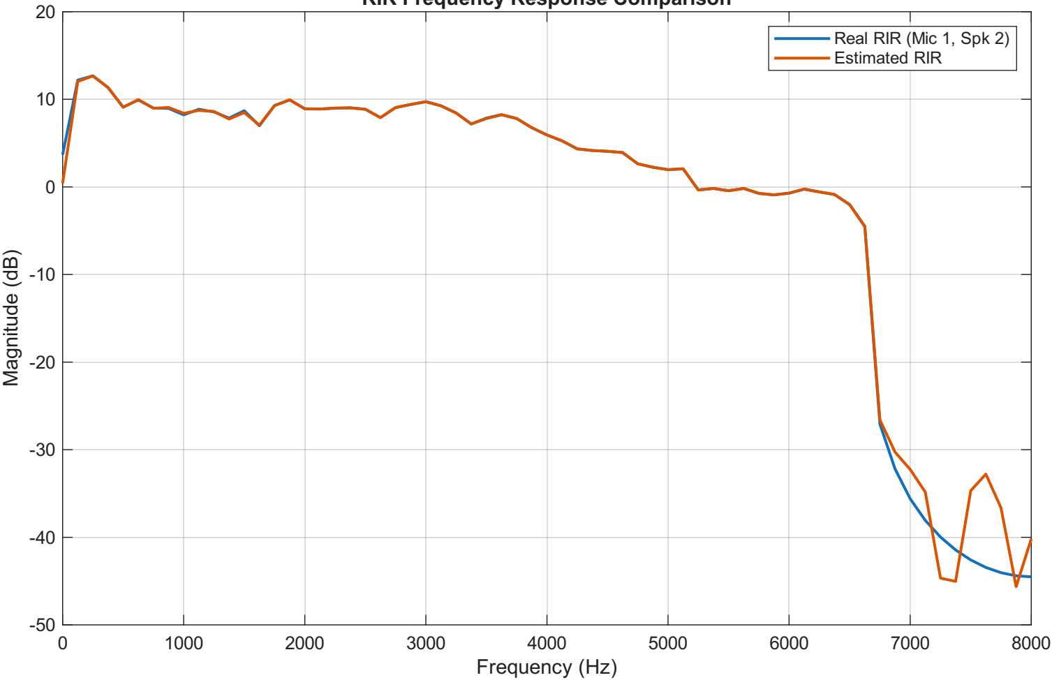
RIR Frequency Response Comparison
