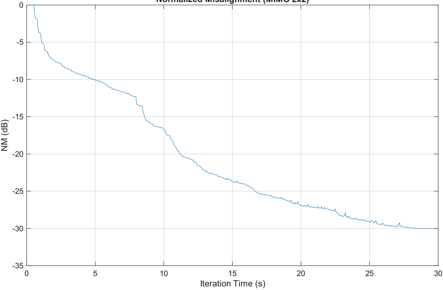
Normalized Misalignment (MIMO 2x2)
