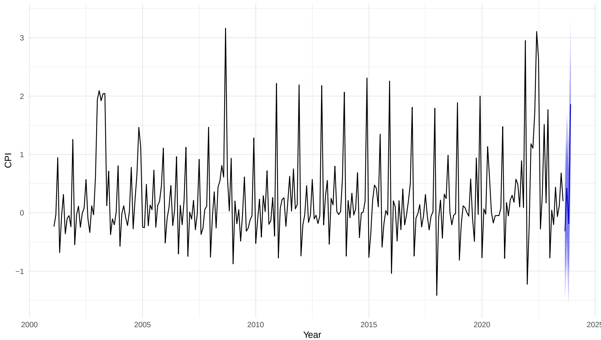
Holt-Winters Additive Model Forecast
