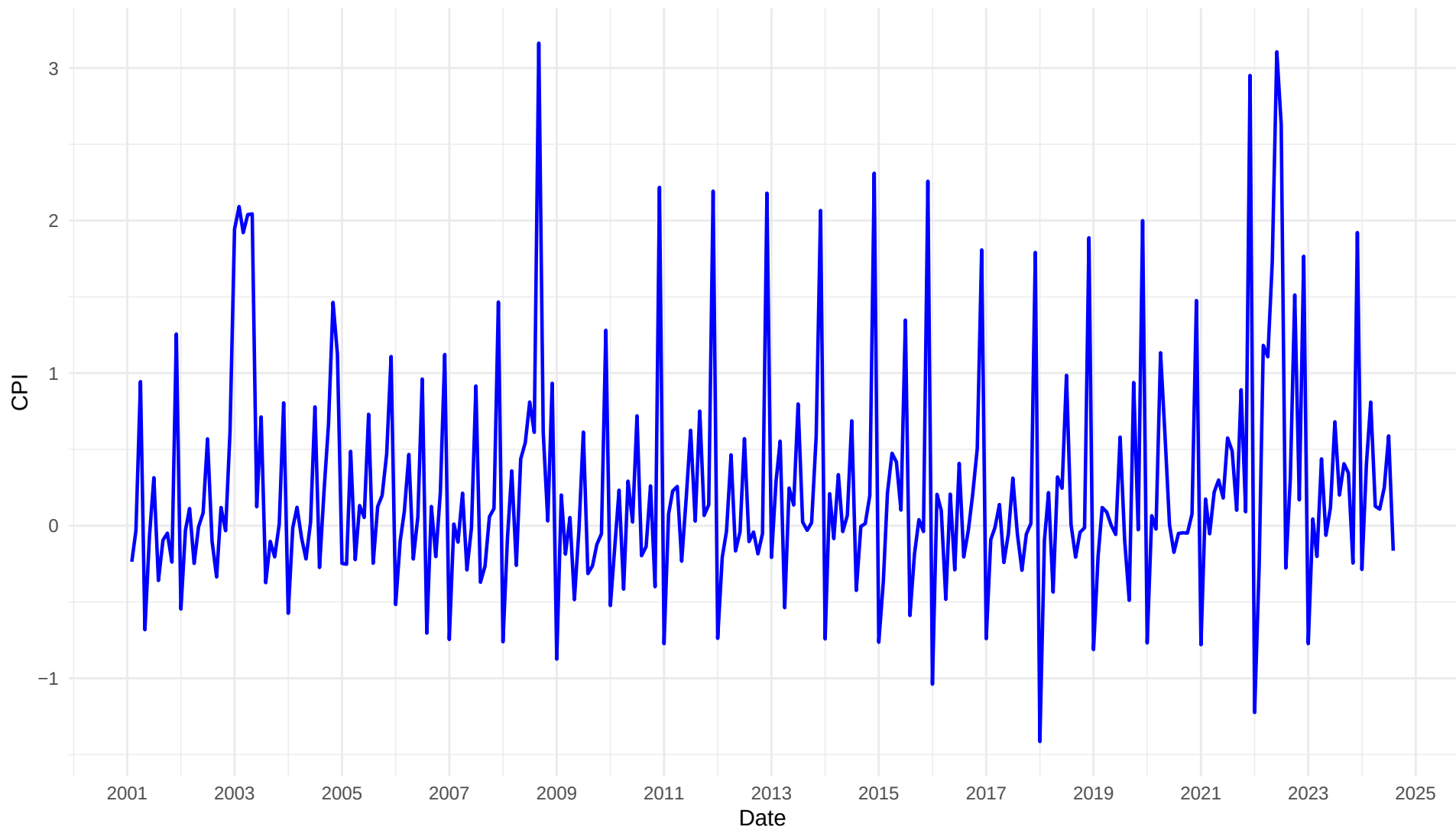
Transport CPI with Smoothing Applied
