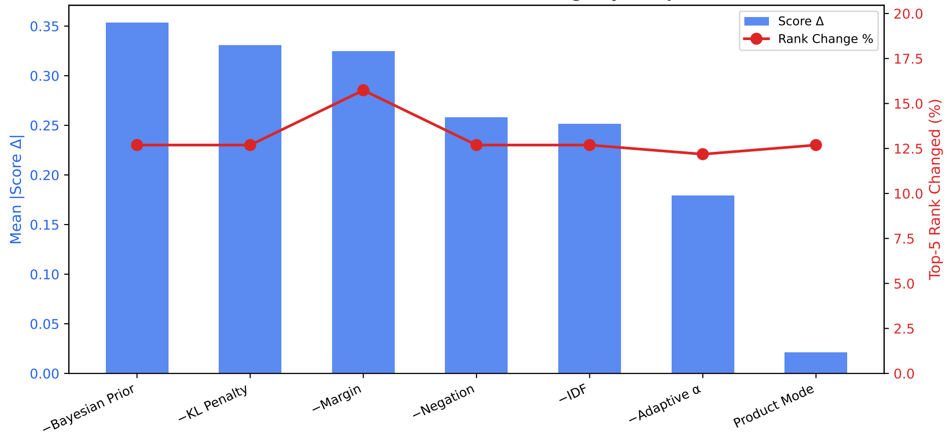
RQ6: Score Perturbation vs Rank Change by Component
