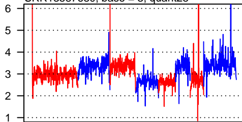
SRR13587680, base = 3, quant25
