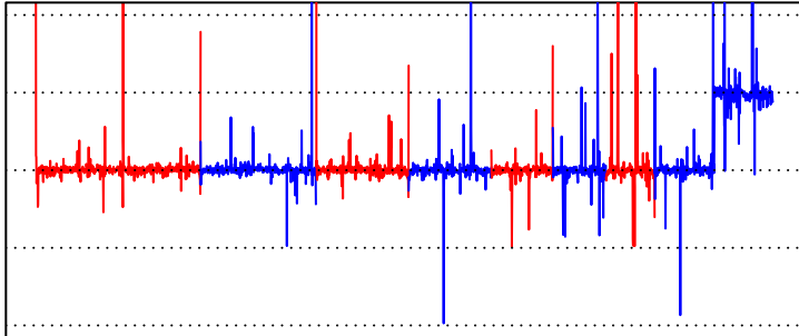
SRR13587806
