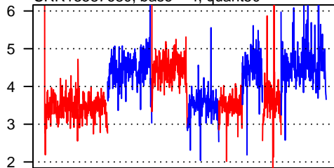
SRR13587680, base = 4, quant50
