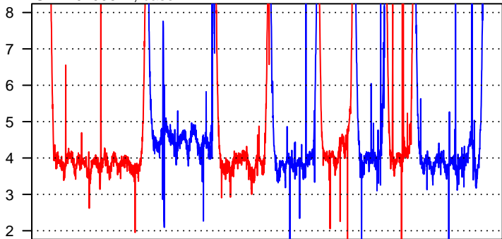
SRR10209617, base = 4
