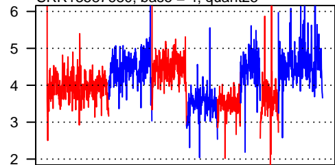
SRR13587680, base = 4, quant25
