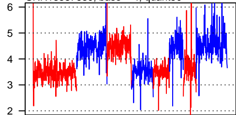
SRR13587680, base = 4, quant50
