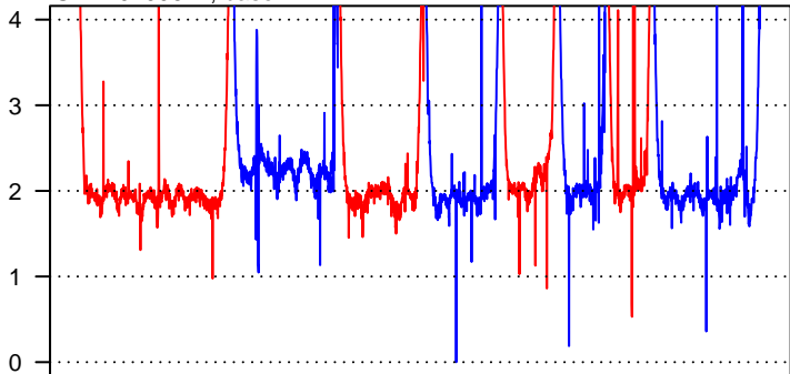
SRR10209617, base = 3
