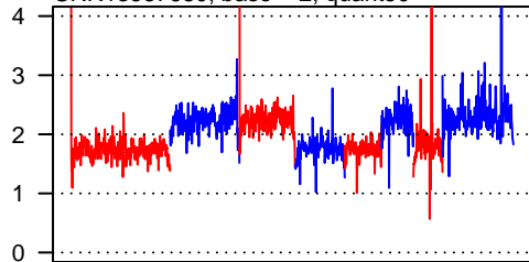
SRR13587680, base = 2, quant50
