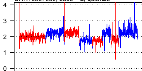
SRR13587680, base = 2, quant25
