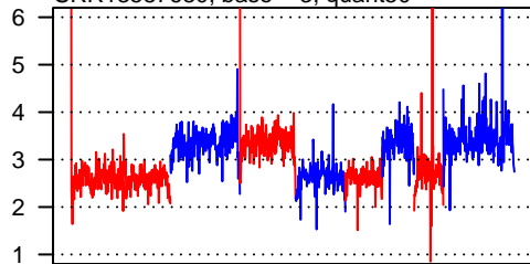
SRR13587680, base = 3, quant50
