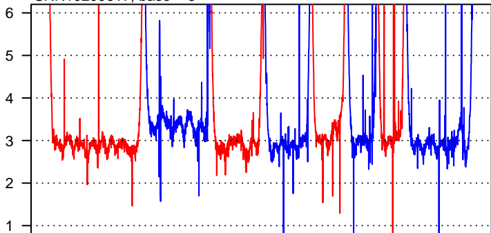
SRR10209617, base = 3
