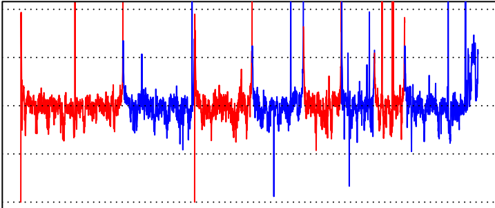
SRR13587818
