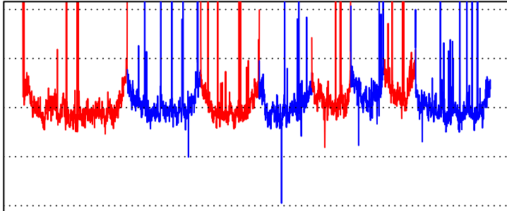
SRR9073715
