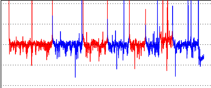
SRR1554302
