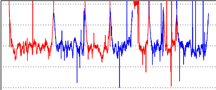
SRR21359704
