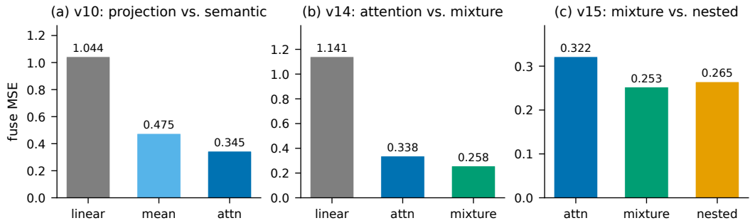
Figure 2: The alignment ladder. (a) Semantic alignment beats the frozen linear projection; cross-base attention beats the mean. (b) The mixture aligner improves on single-concept attention. (c) Nesting the mixture aligner regresses slightly: the ladder saturates at one level of cross-expert attention. Lower is better.
