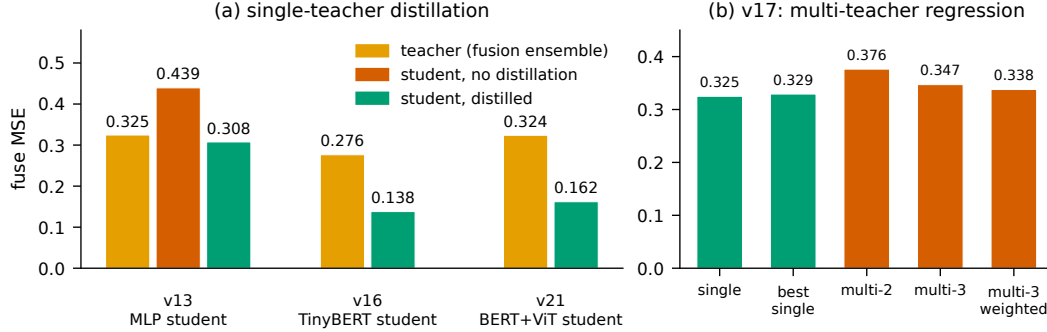
Figure 3: (a) Single-teacher chimera distillation: distilled students beat their multi-base teacher in every setting. (b) Multi-teacher distillation regresses across all configurations (v17). Lower is better.
