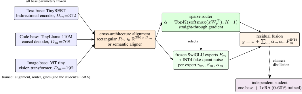
Figure 1: Heterogeneous micro-fusion and chimera distillation. Three frozen pretrained bases with different architectures and hidden widths are natively encoded, aligned into a shared 256-dimensional space, and sparsely routed ( K=1 ) to frozen SwiGLU experts whose outputs carry INT4 fake-quantization noise. Chimera distillation then collapses the ensemble into one independent single-base student.
