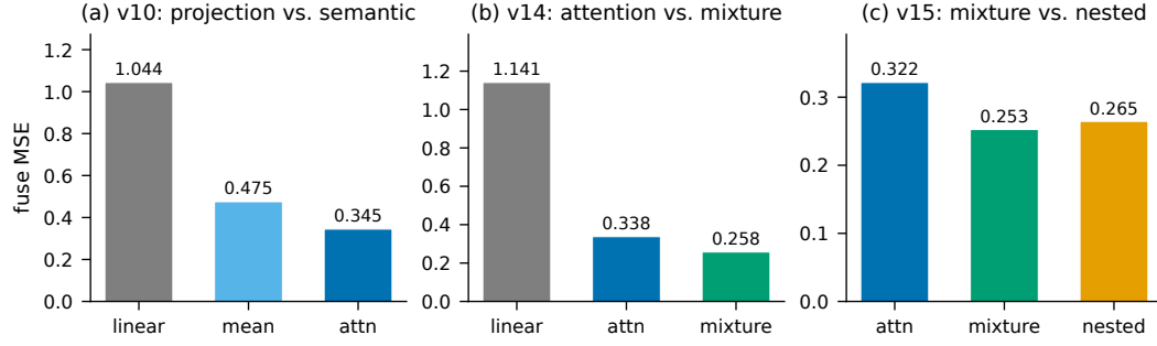
Figure 5: The alignment ladder. (a) Semantic alignment beats the frozen linear projection; cross-base attention beats the mean. (b) The mixture aligner improves on single-concept attention. (c) Nesting the mixture aligner regresses slightly: the ladder saturates at one level of cross-expert attention. Lower is better.
