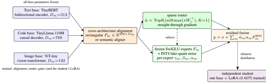
Figure 2: Heterogeneous micro-fusion and chimera distillation. Three frozen pretrained bases with different architectures and hidden widths are natively encoded, aligned into a shared 256-dimensional space, and sparsely routed ( K=1 ) to frozen SwiGLU experts whose outputs carry INT4 fake-quantization noise. Chimera distillation then collapses the ensemble into one independent single-base student.
