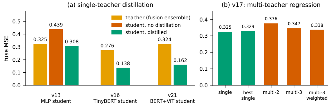
Figure 6: (a) Single-teacher chimera distillation: distilled students beat their multi-base teacher in every setting. (b) Multi-teacher distillation regresses across all configurations (v17). Lower is better.
