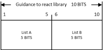
Figure 4.2-4 Format of the Guidance to react library Field (DCX message (information from organizations outside Japan))
