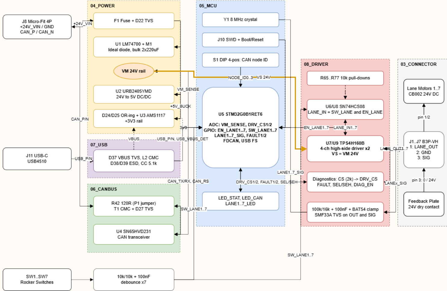
HW_ADHERENT_LANECTRL_R1 - Block / Signal Flow Diagram
