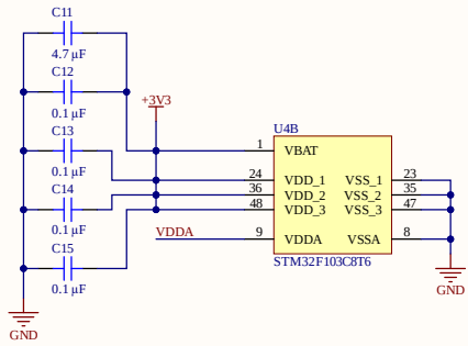
STM32 POWER
