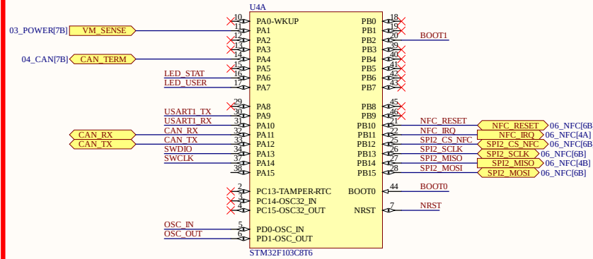
STM32F103C8T6 MCU
