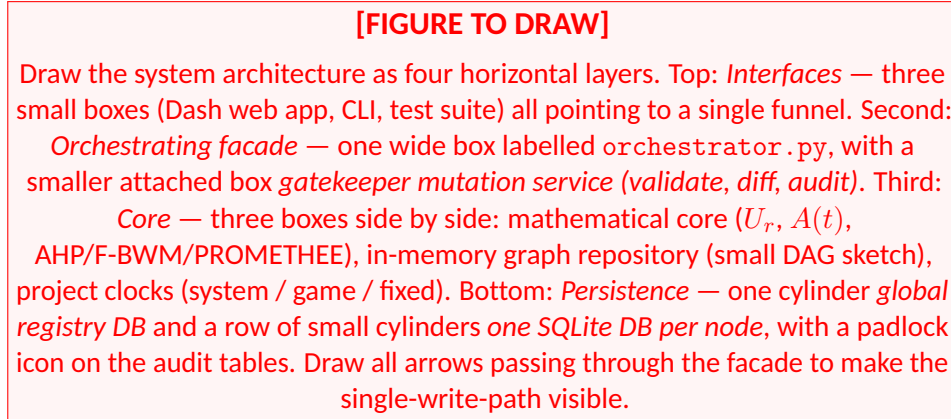
Figure 6: SupplyScore system architecture: single facade, gated writes, multi-tenant persistence.
