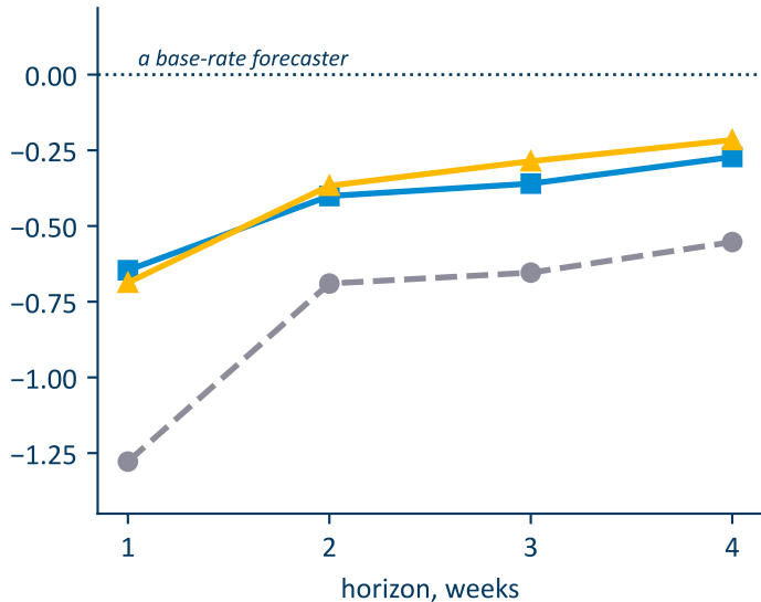
Brier skill
