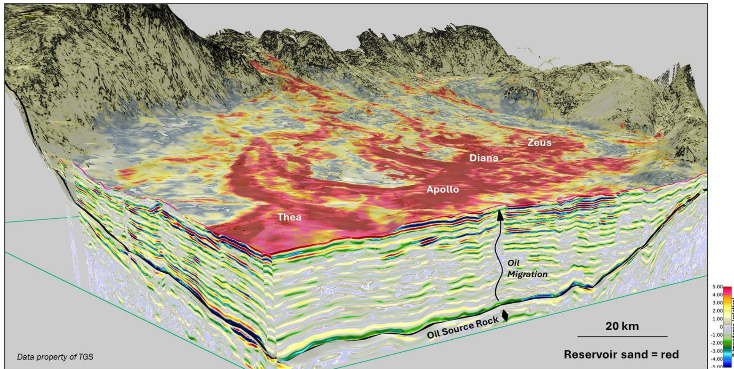
Relative acoustic impedance: Cenomanian top 100 m
