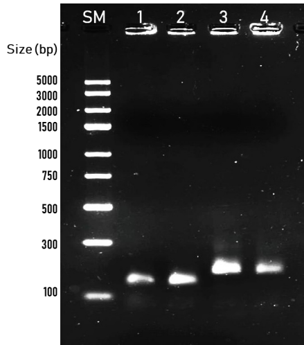
Figure S3. PCR products obtained with insert-specific primers before cloning. SM, GeneRuler Express DNA Ladder; lanes 1–2, A insert; lanes 3–4, B insert.
