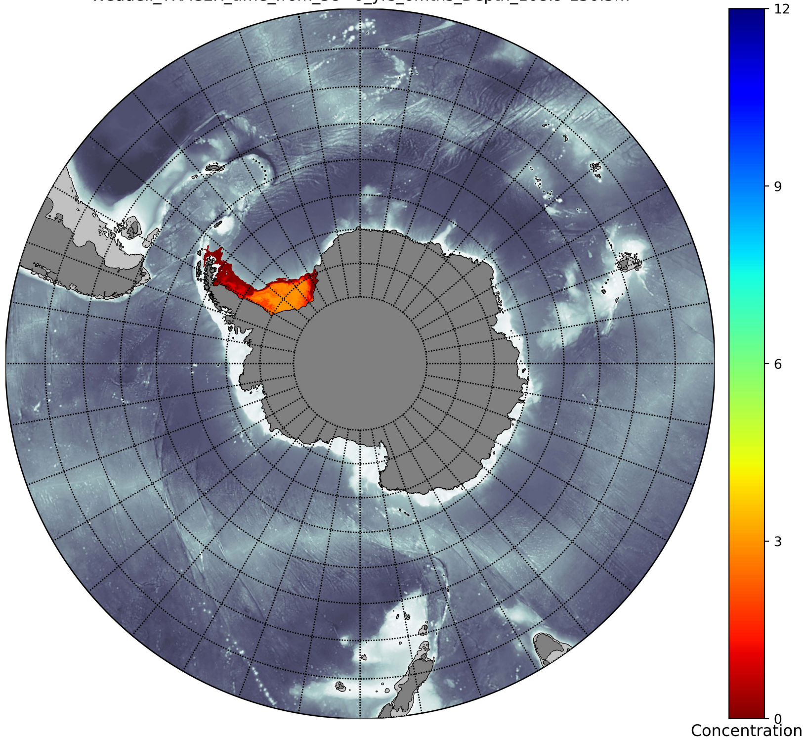
Weddell_TRACER_time_from_58=0_yrs_6mths_Depth_108.9-150.5m
