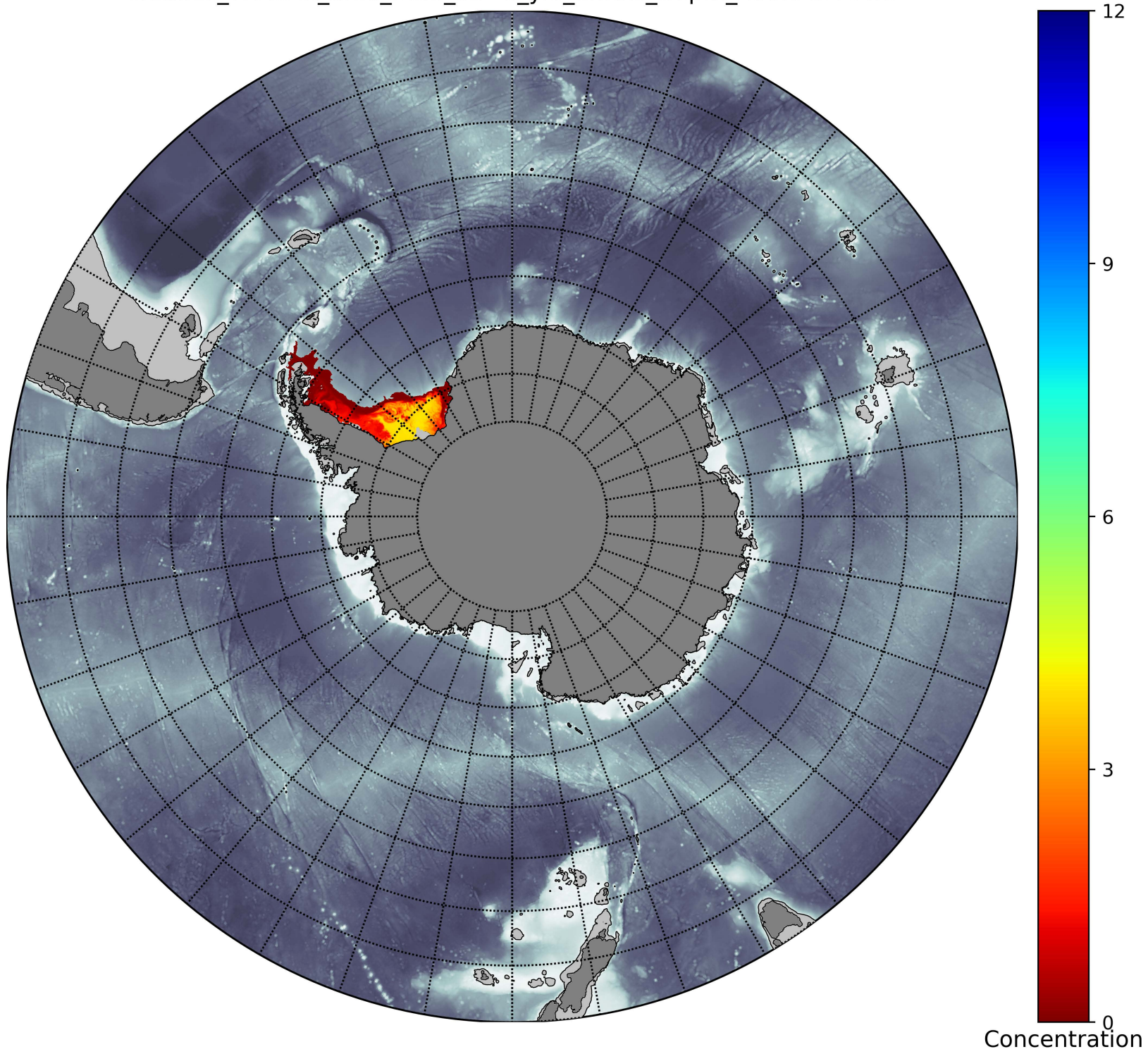
Weddell_TRACER_time_from_58=0_yrs_6mths_Depth_206.6-312.4m
