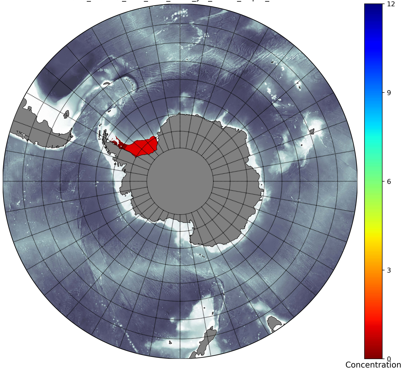
Weddell_TRACER_time_from_58=0_yrs_6mths_Depth_0.0-0.5m
