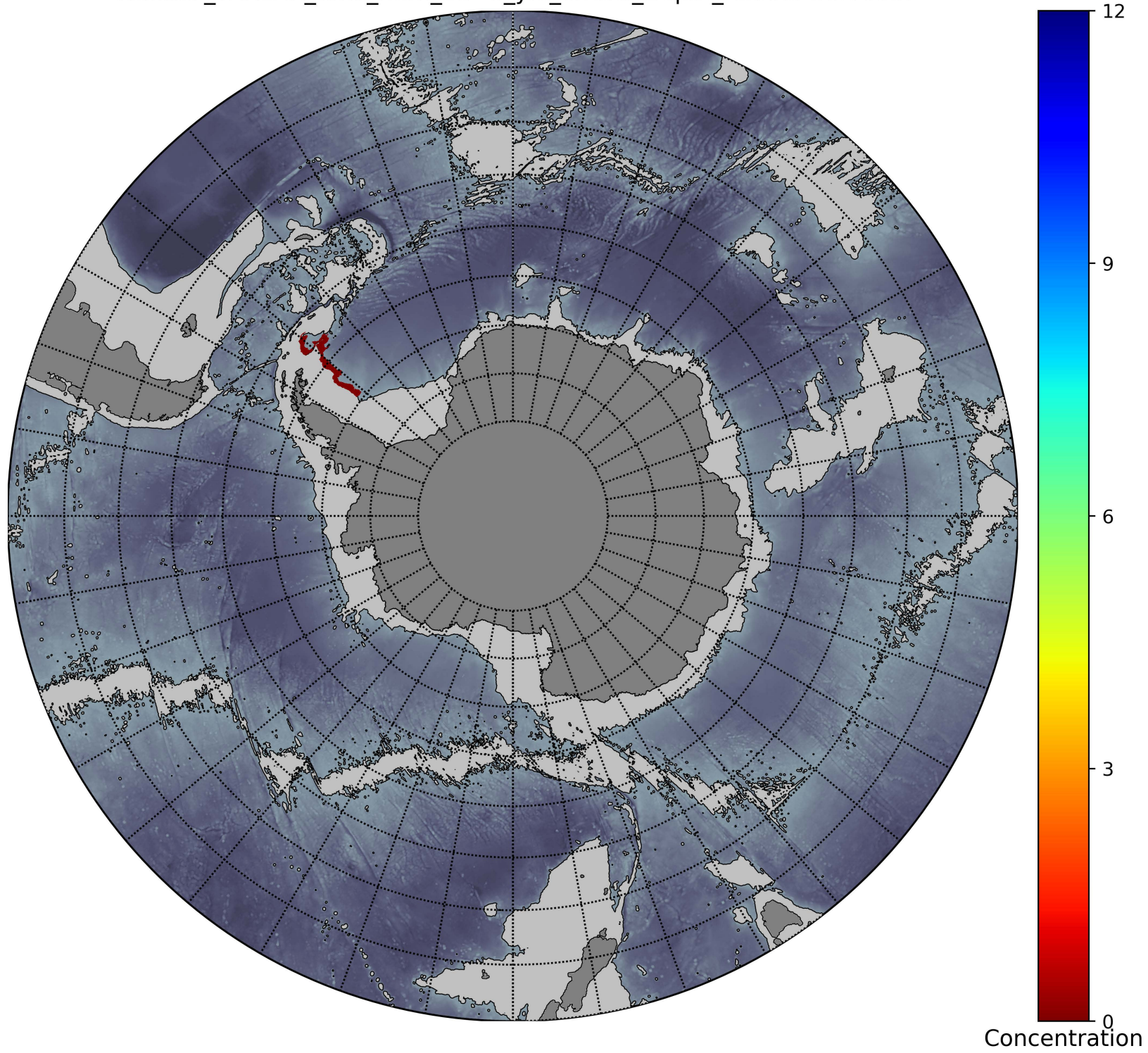
Weddell_TRACER_time_from_58=0_yrs_6mths_Depth_2006.9-3012.6m
