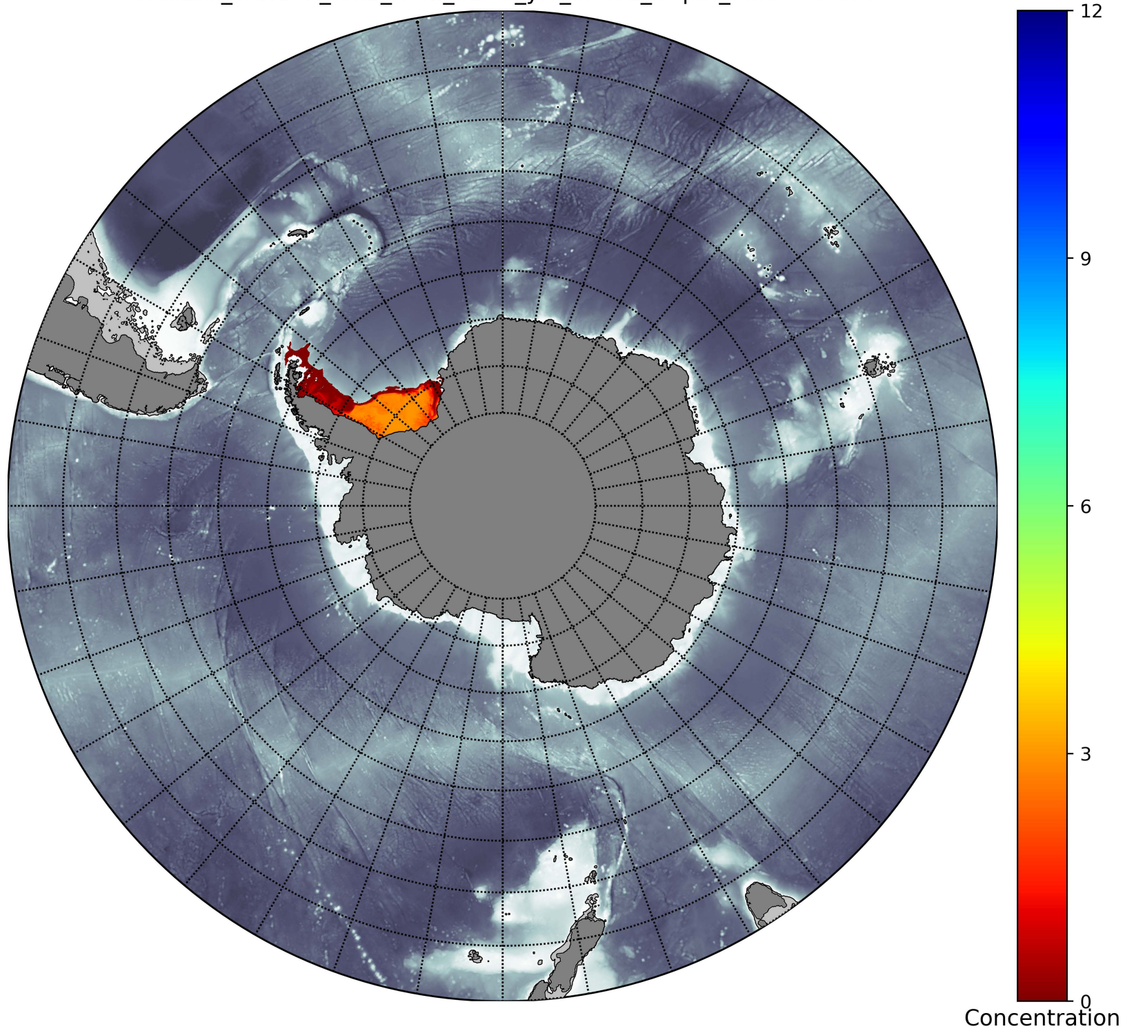
Weddell_TRACER_time_from_58=0_yrs_6mths_Depth_78.0-108.9m
