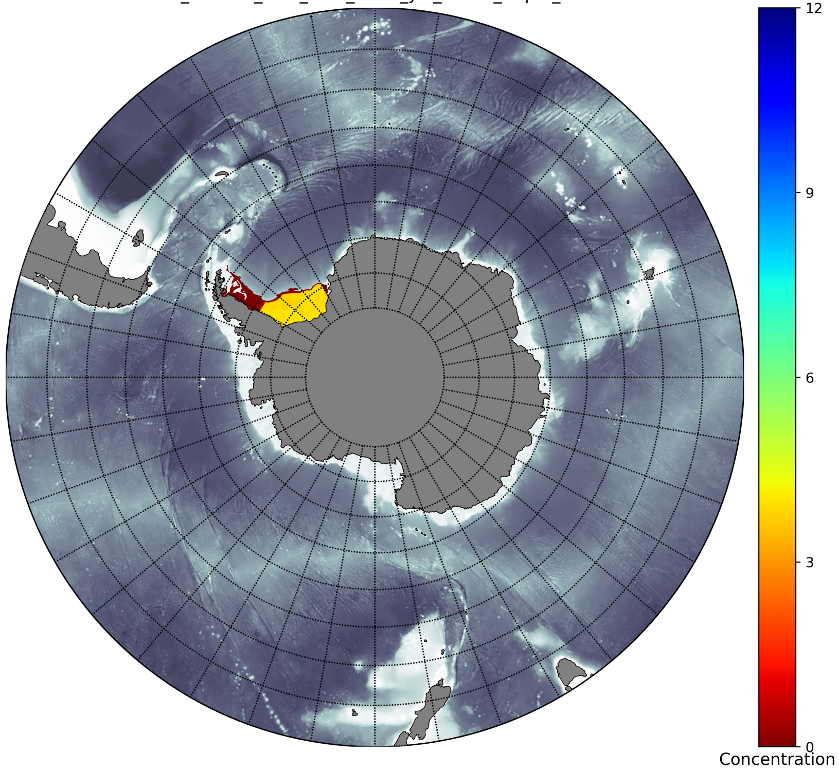
Weddell_TRACER_time_from_58=0_yrs_6mths_Depth_0.5-5.8m
