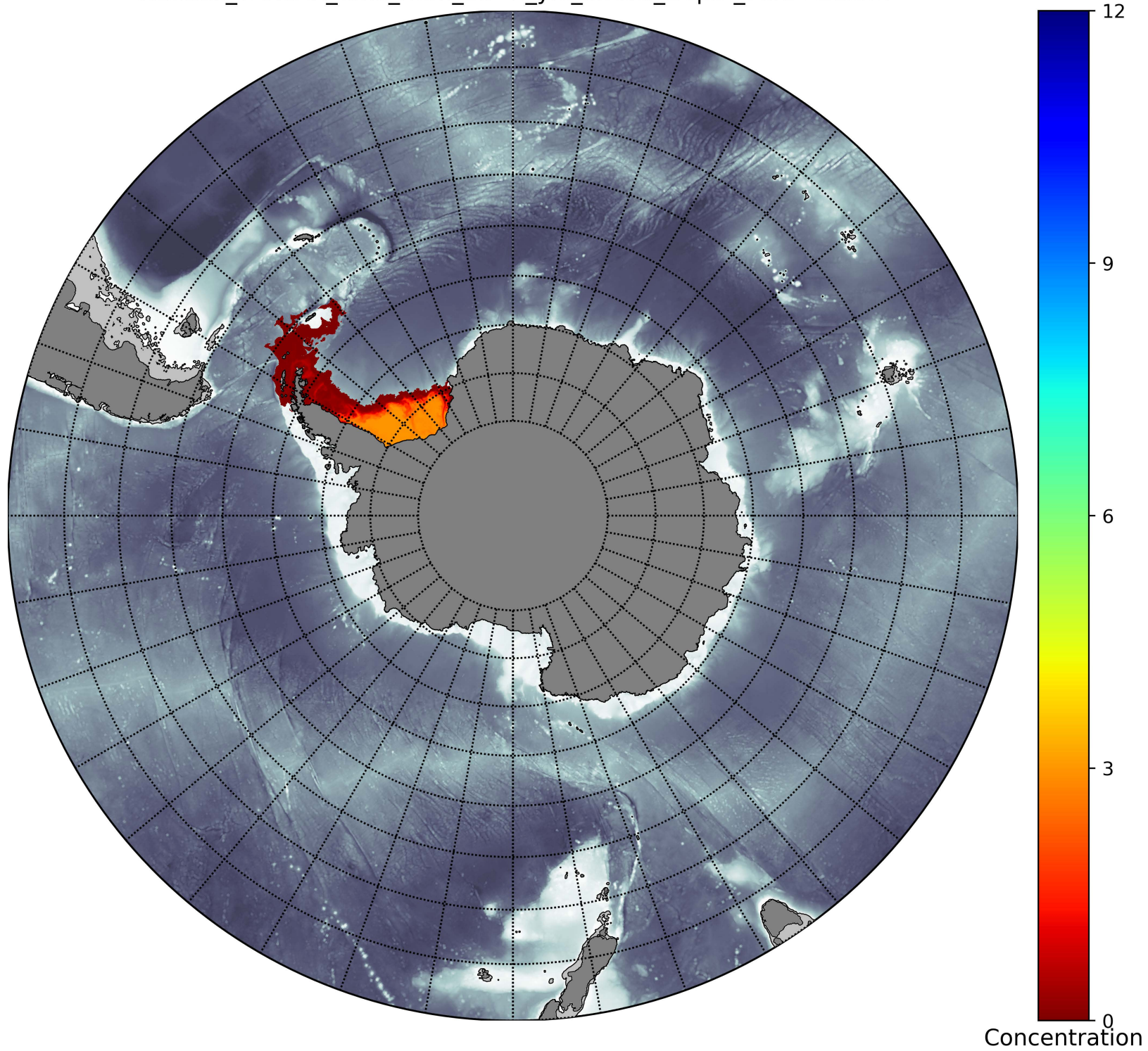
Weddell_TRACER_time_from_58=2_yrs_0mths_Depth_78.0-108.9m
