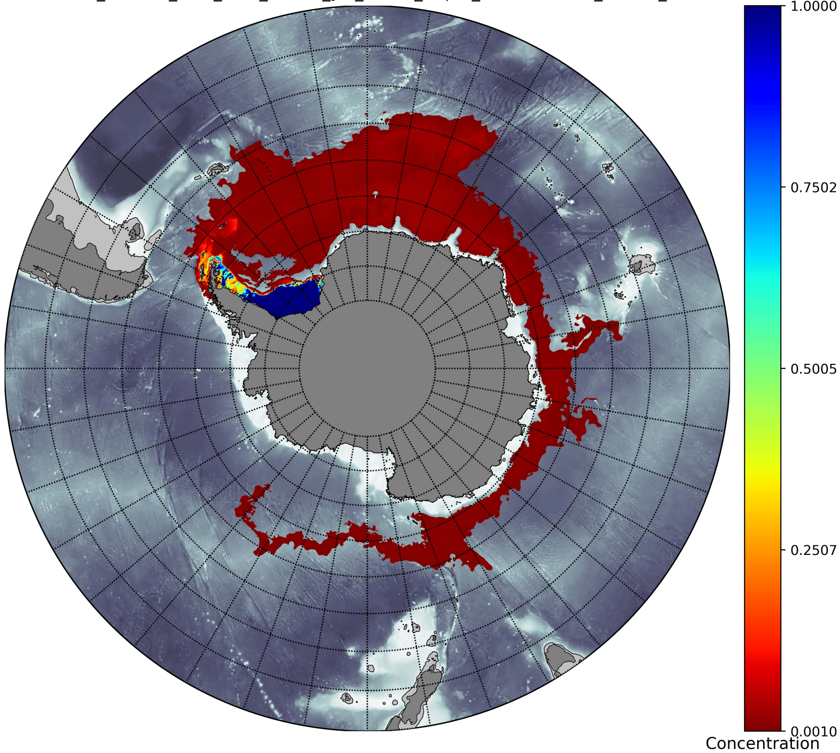
Weddell_TRACER_time_from_58=30_yrs_0mths_Depth_150.5-206.6m_narrow_cbar
