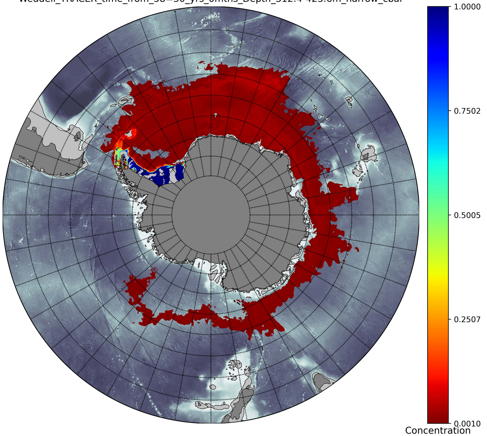
Weddell_TRACER_time_from_58=30_yrs_0mths_Depth_312.4-423.6m_narrow_cbar
