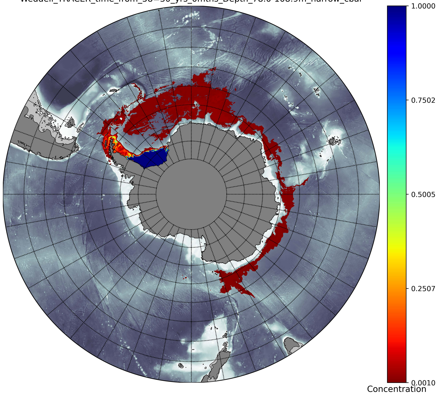
Weddell_TRACER_time_from_58=30_yrs_0mths_Depth_78.0-108.9m_narrow_cbar
