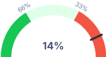
Compression Rate
