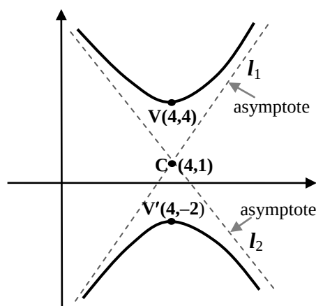
Figure 4.29: \frac{(y-1)^2}{9} - \frac{(x-4)^2}{4} = 1
