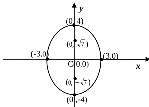
Figure 4.20: 16x^2 + 9y^2
