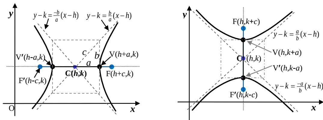
Figure 4.27: (a) Horizontal hyperbola with center C(h,k)
