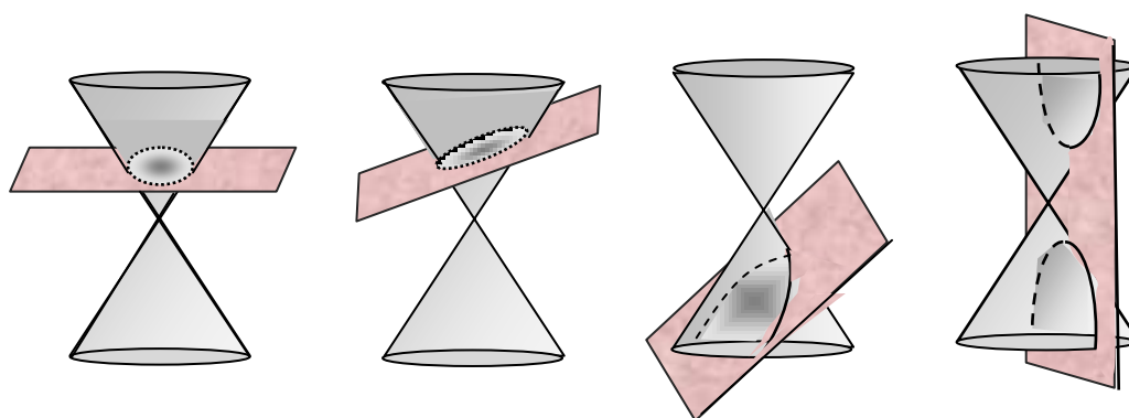
Figure 4.1: (a) circle
