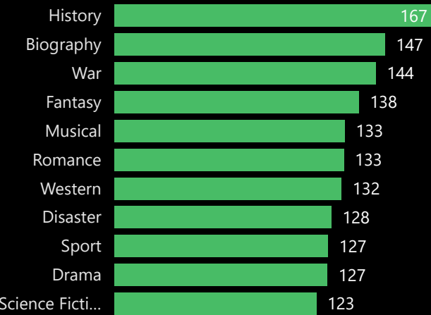
Average Runtime
