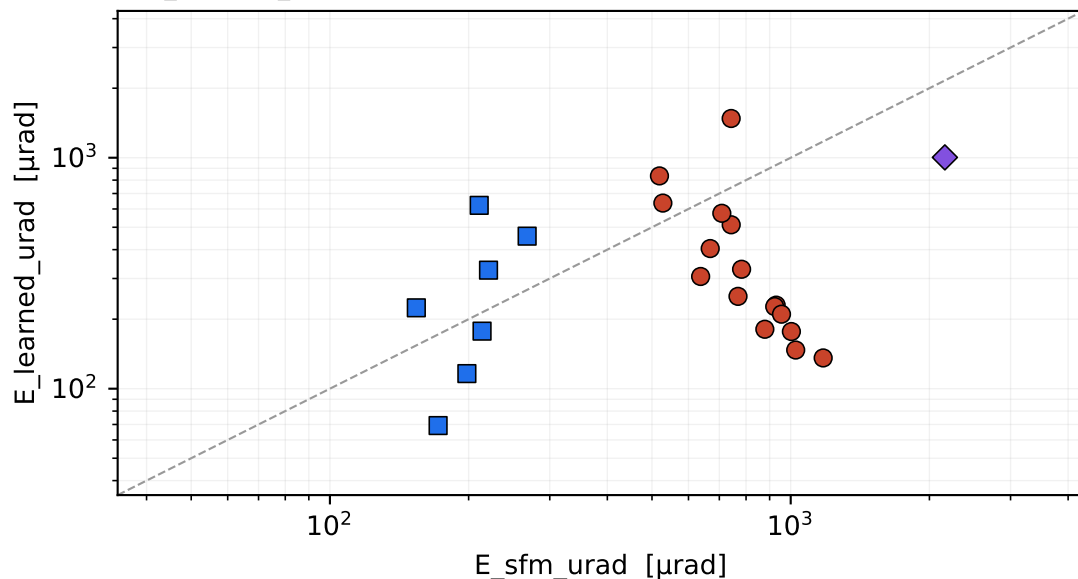
A. E_sfm vs E_learned \rho = -0.05 ( p = 0.824 , n = 24 )
