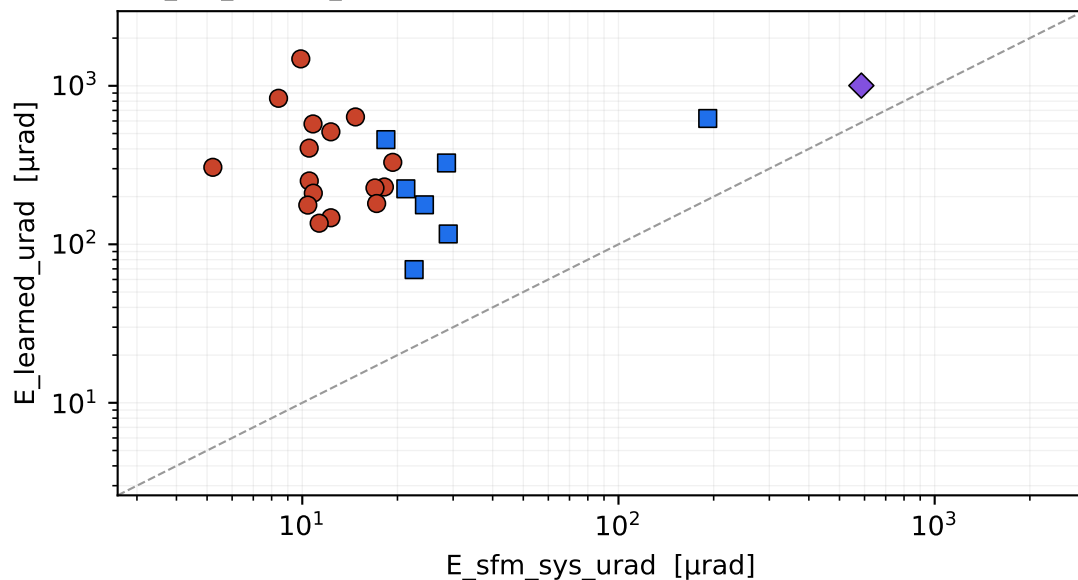
C. E_sfm_sys vs E_learned \rho = -0.15 ( p = 0.470 , n = 24 )
