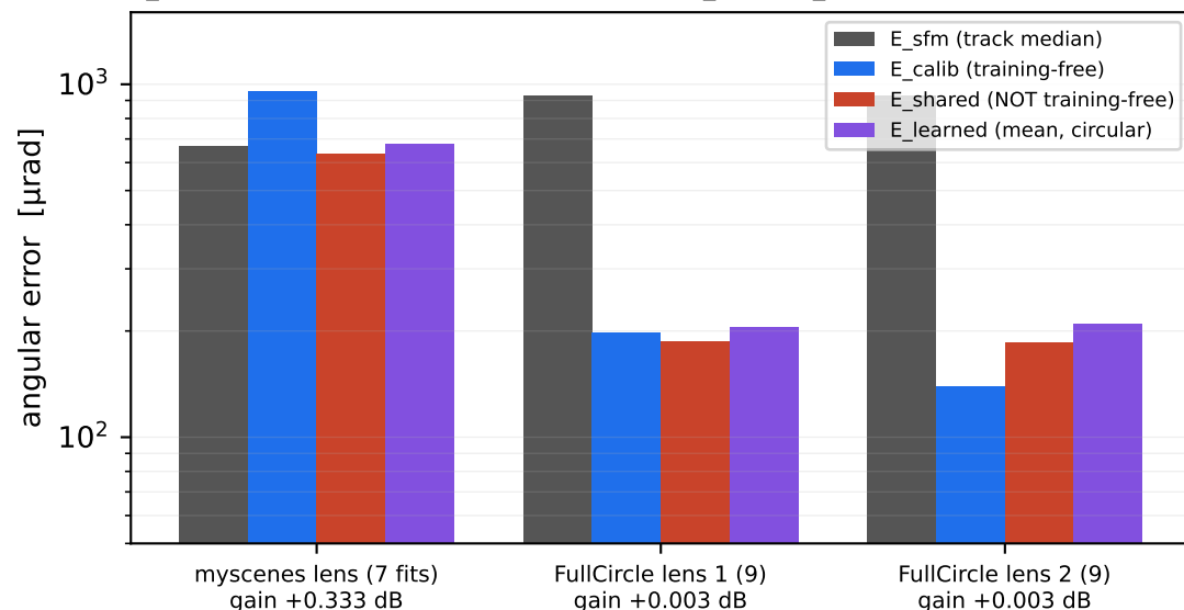
D. The three lenses where E_shared exists at all ( \geq 3 fits of one glass). E_sfm orders them BACKWARDS vs the gain; E_calib / E_shared order them correctly.
