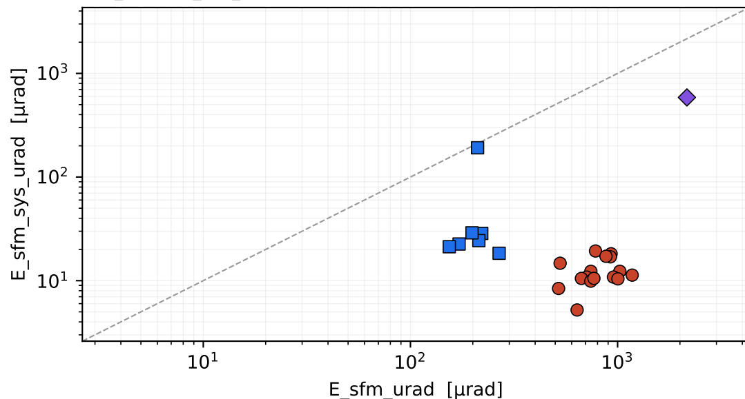
B. E_sfm vs E_sfm_sys \rho = -0.31 ( p = 0.139 , n = 24 )
