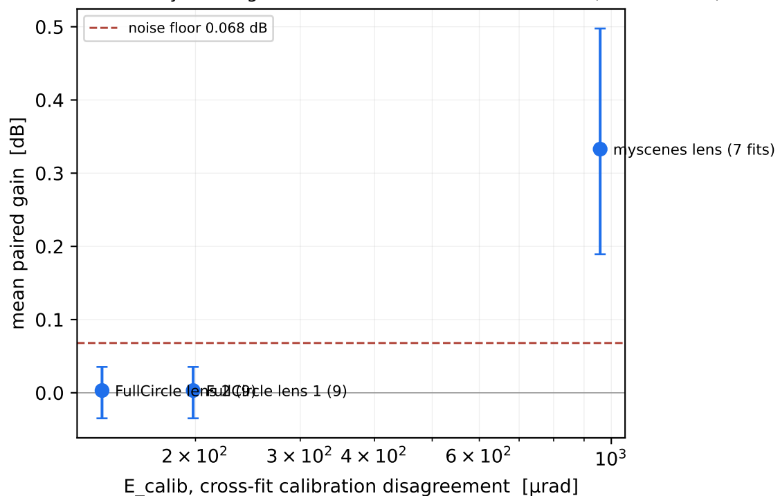
B. The only training-free statistic that orders the tracks ( n = 3 lenses)
