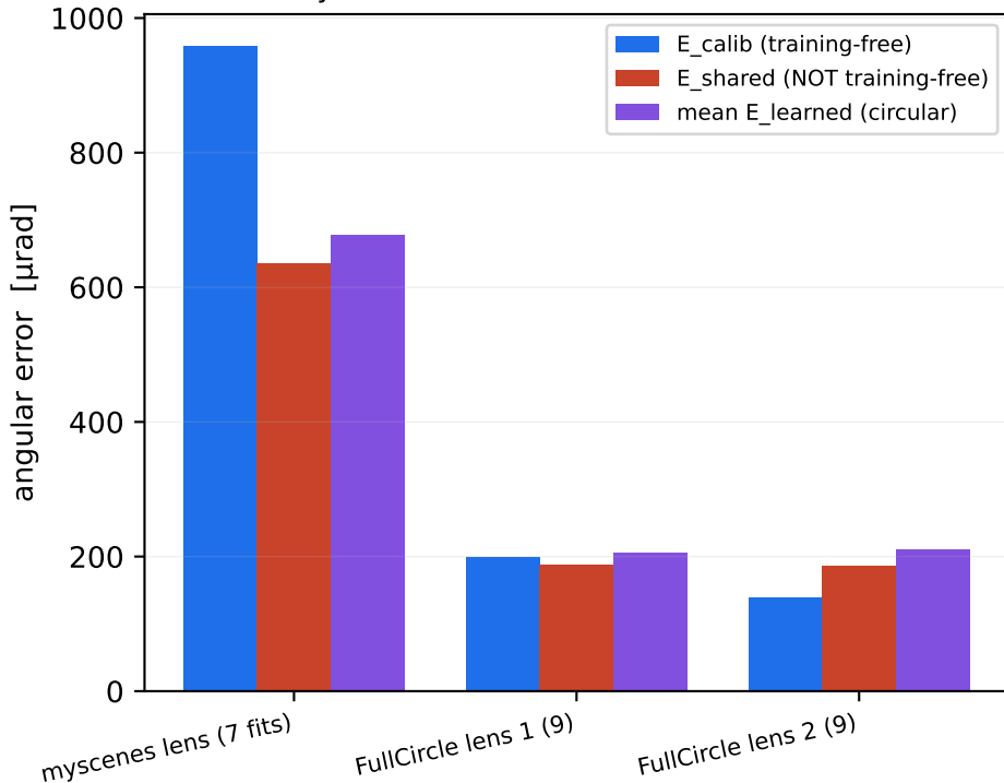
A. Three ways to size the same lens's calibration error
