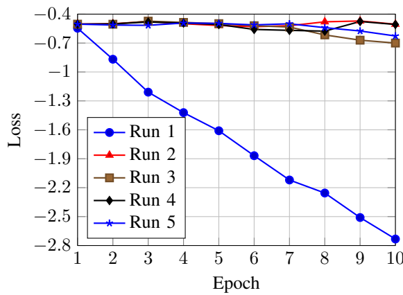
Training Progress vs. Loss (Torch_conv_hybrid_quantum)
