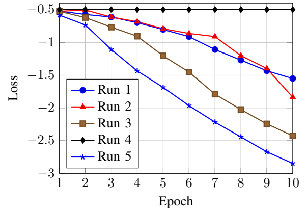
Training Progress vs. Loss (custom model)
