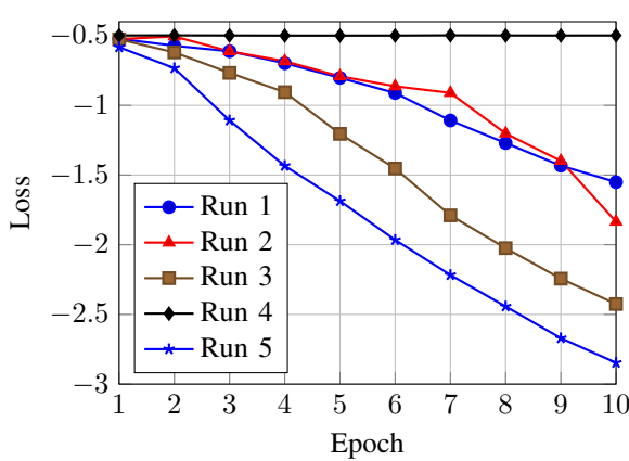
Training Progress vs. Loss (custom model)
