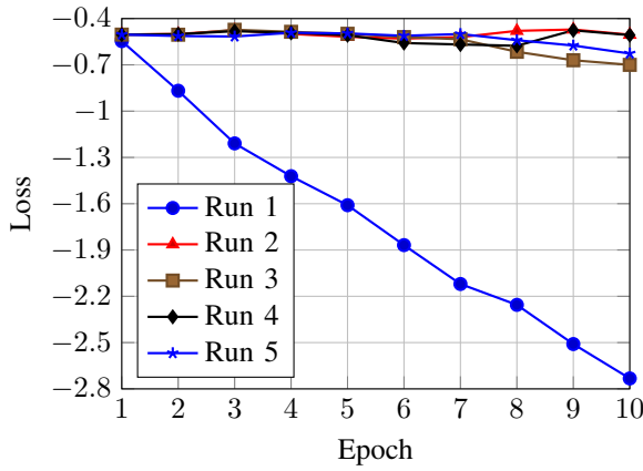
Training Progress vs. Loss (Torch_con_nd_hybrid_qnn.py)
