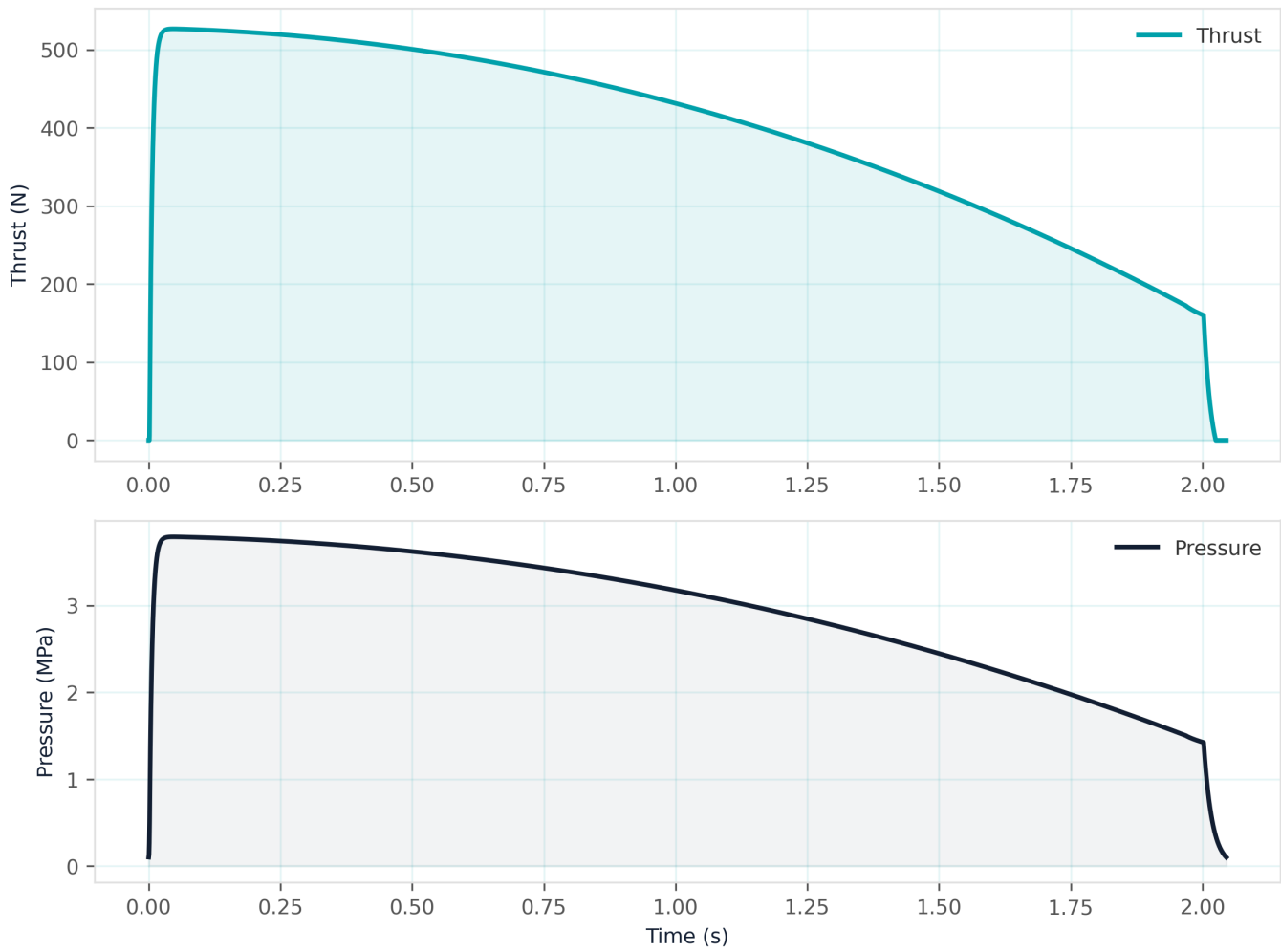
Summary: Class J motor delivering 803 Ns with a peak thrust of 527 N.
