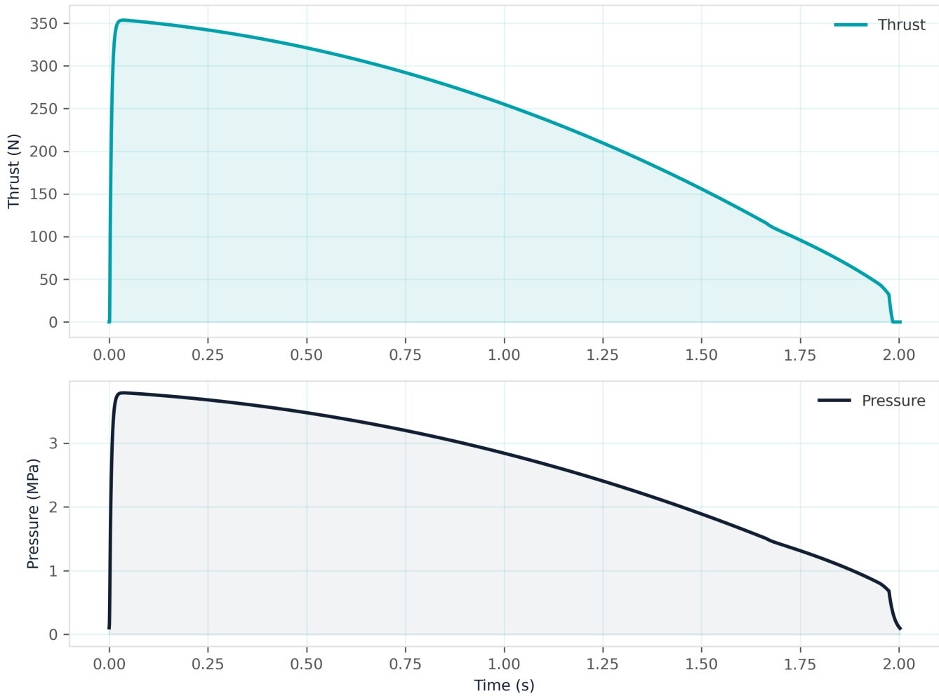
Summary: Class I motor delivering 465 Ns with a peak thrust of 354 N.
