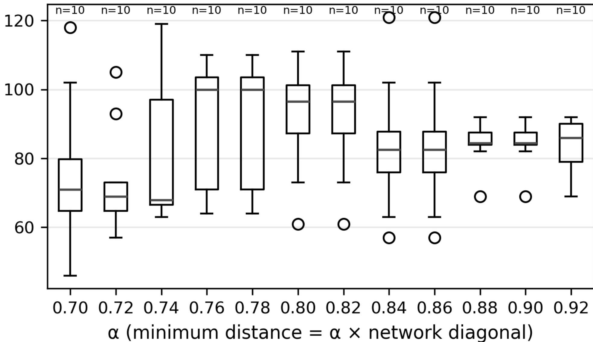
Distribution of free-flow shortest-path travel times (Sioux_Falls.net)
