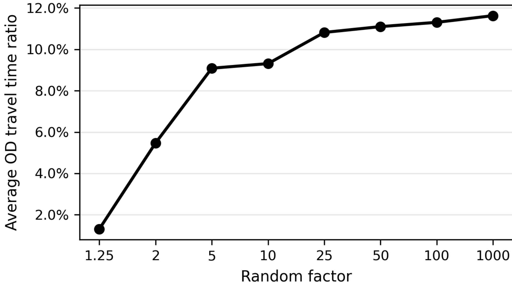
Effect of random factor on route set quality
