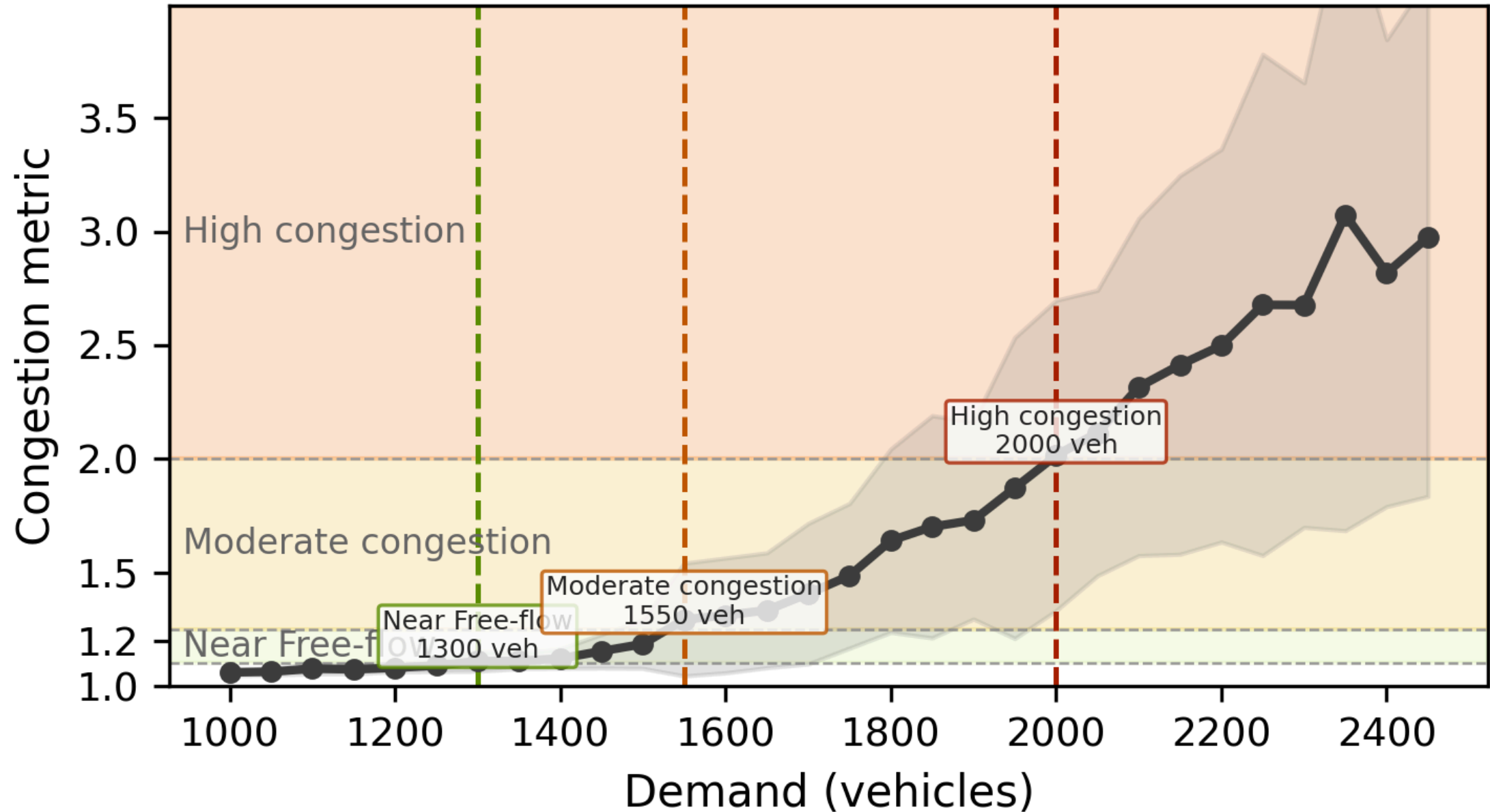
Congestion metric vs demand (Sioux_Falls.net)
