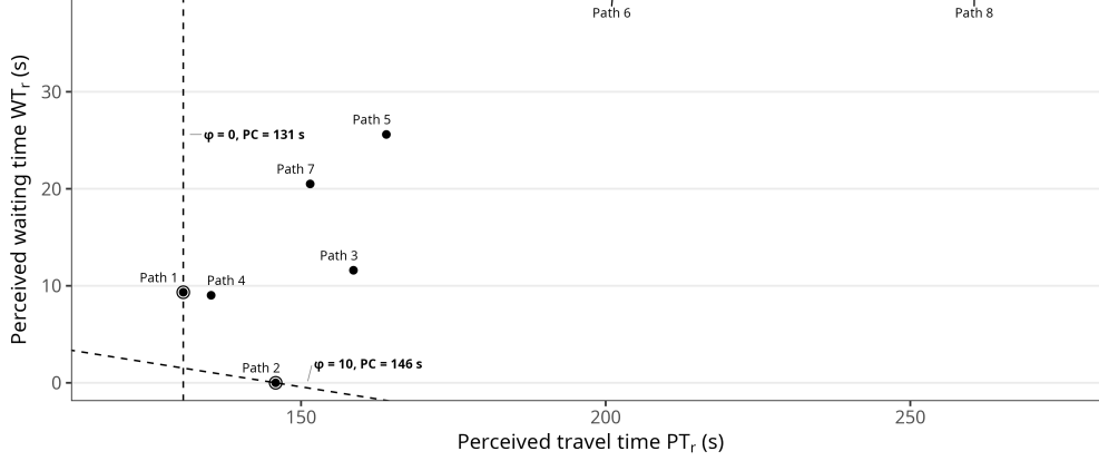
FIG. 37. Illustration of the effect of waiting-time sensitivity on perceived route costs for a representative agent. Highlighted points indicate the minimum-cost route for \varphi = 0 and \varphi = 10 , while dashed lines indicate equal perceived cost, where perceived route cost is calculated as PT_r + \varphi \cdot WT_r . The reported perceived route costs correspond to the final episode of a scenario without waiting-time-sensitive drivers.
