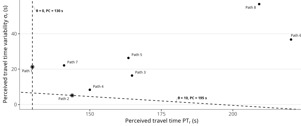
FIG. 33. Illustration of the effect of risk sensitivity on perceived route costs for a representative agent and random seed. Highlighted points indicate the minimum-cost route for \theta = 0 and \theta = 10 , while dashed lines indicate equal perceived cost, where the perceived route cost is calculated as PT_r + \theta \cdot \sigma_r . The reported perceived route costs correspond to the final episode of a scenario without risk-sensitive drivers.
