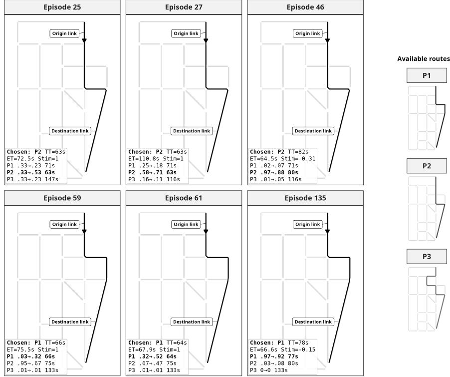
FIG. 26. Evolution of route choice for a representative agent with memory level 0.1 under a high congestion scenario. The panels show the selected route and an annotation box containing the ID of the chosen route and the corresponding experienced travel time, expected travel time (ET), stimulus, route-choice probabilities, and perceived travel times (PT) of each route for that episode. The right sidebar shows the routes available to the representative agent. Regarding the notation for route-choice probabilities, for example, P1 .33 \rightarrow .23 indicates that the probability of choosing P1 (path 1) decreases from 0.33 to 0.23 during the agent's policy update.
