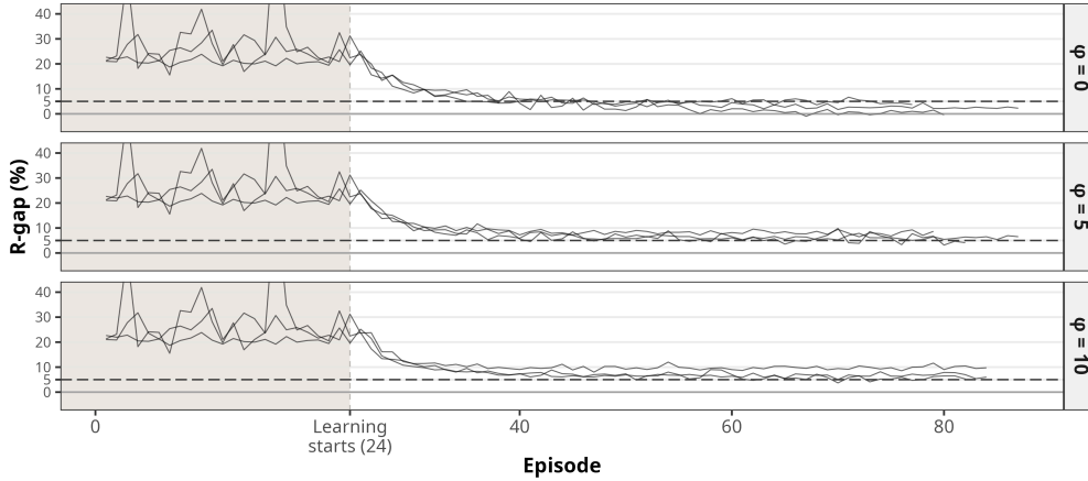
FIG. 38. Effect of different levels of waiting-time sensitivity on R-gap convergence across three representative random seeds.
