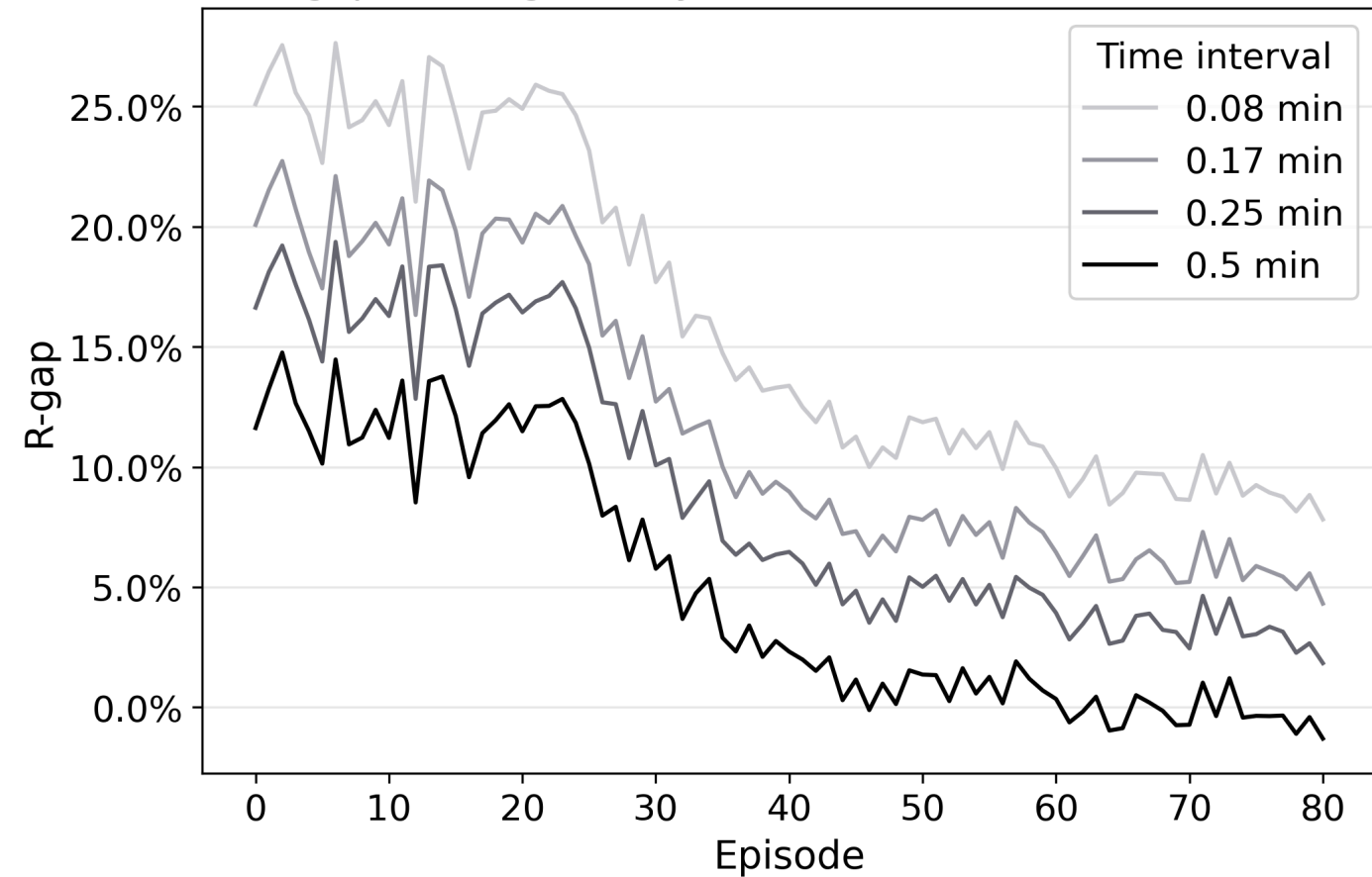
R-gap convergence by time interval (demand = 1550)
