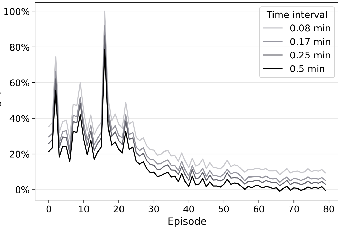
R-gap convergence by time interval (demand = 2000)
