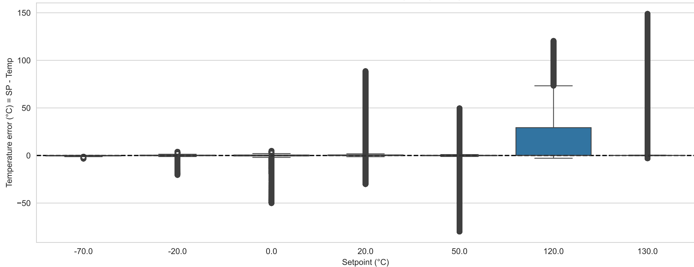
Error Distribution per Setpoint (steady-state)
