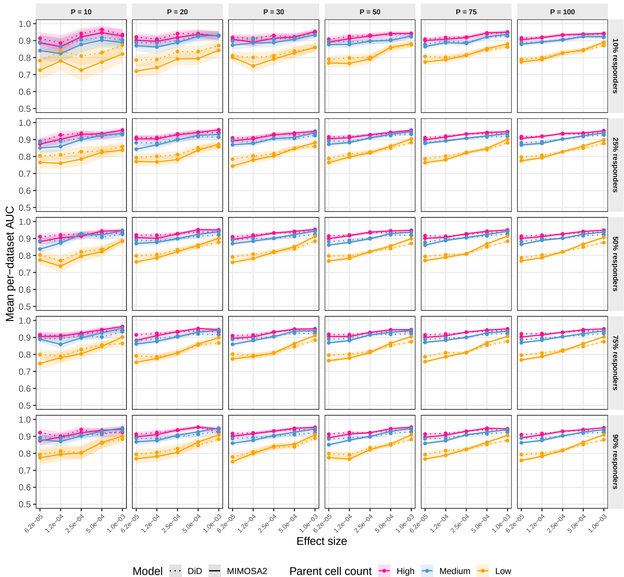
Discrimination of MIMOSA2 and DiD. AUC computed within each dataset, then averaged.
