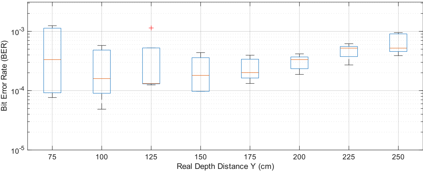
BER Dispersion across Depths Y ( 1/P_n = -28.0 dB)
