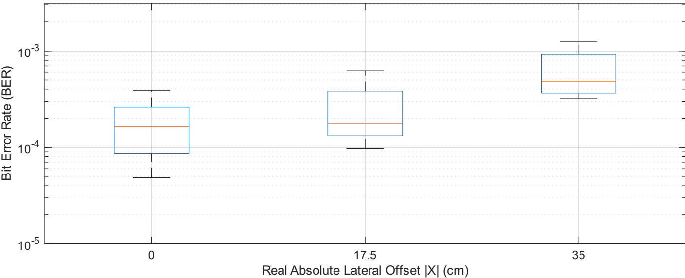
BER Dispersion across Symmetrized Offsets |X| ( 1/P_n = -28.0 dB)
