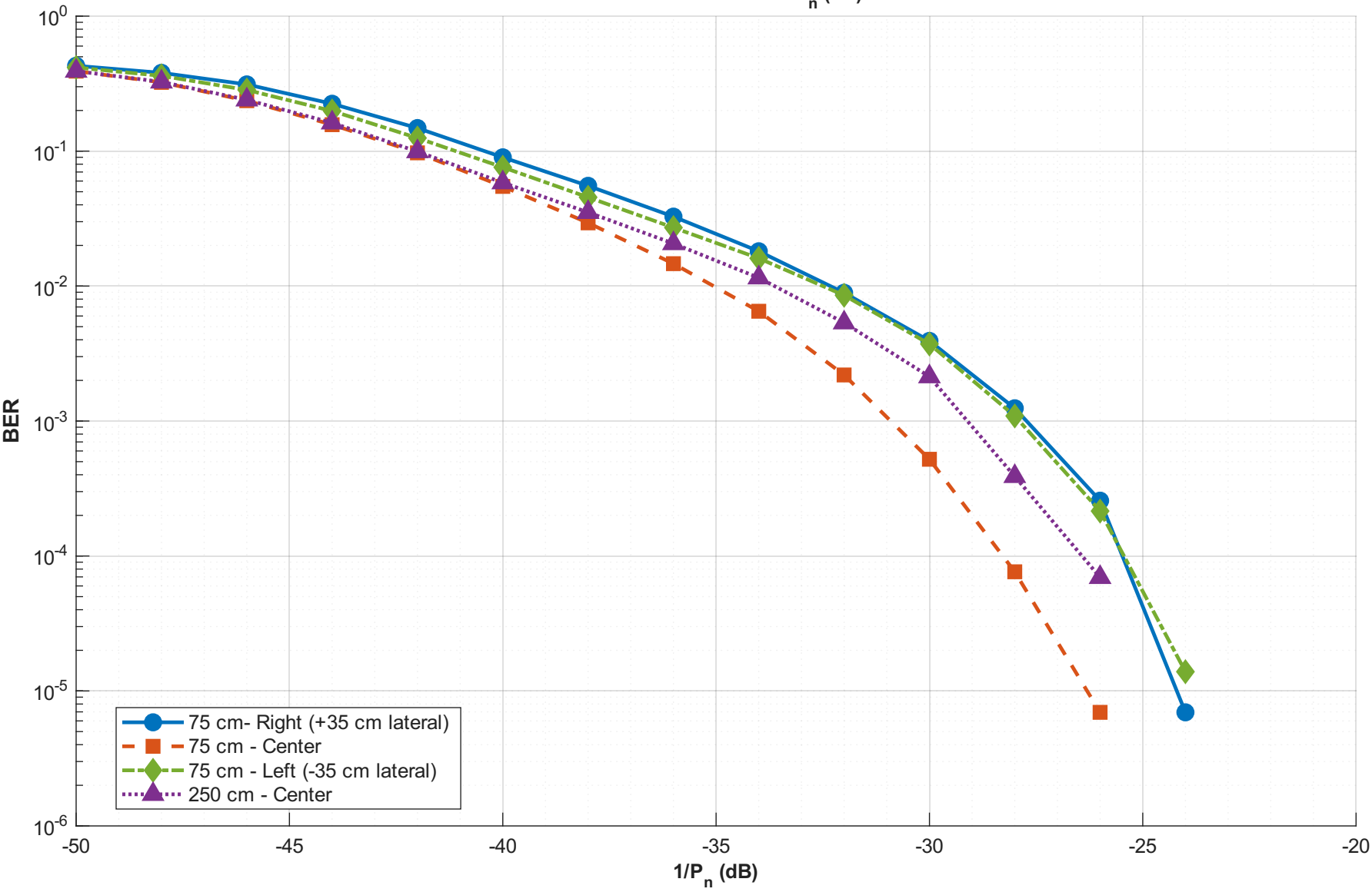
BER Performance vs. 1/P_n (dB)
