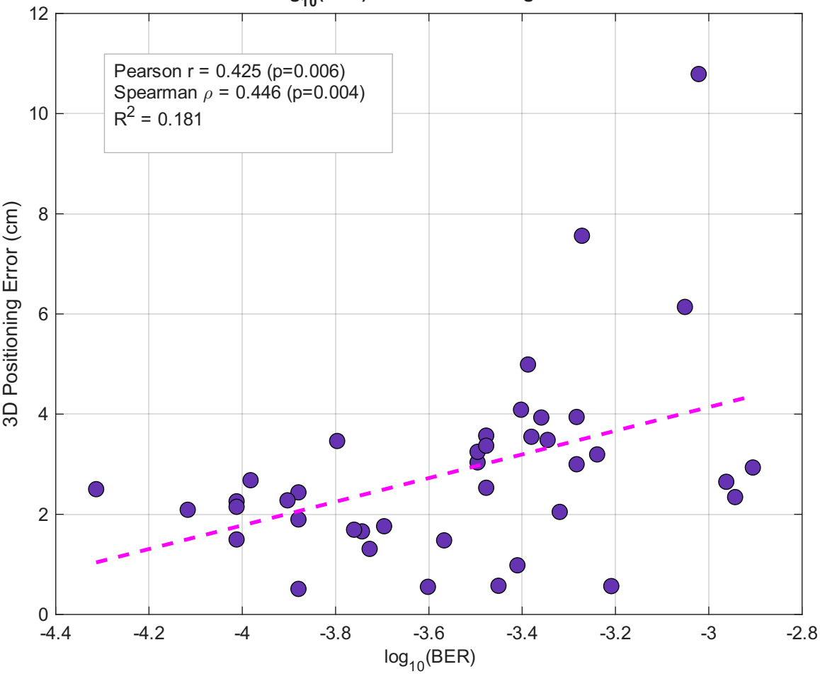
\log_{10}(\text{BER}) vs. 3D Positioning Error
