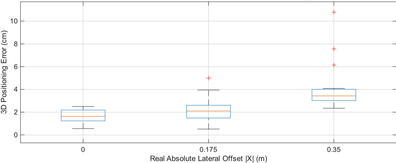
3D Error Dispersion across Symmetrized Lateral Offsets |X|
